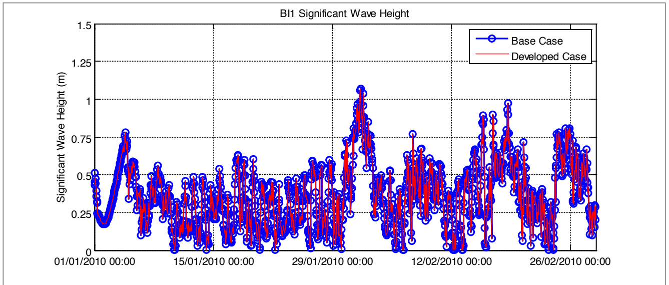
Figure B1: Wave impacts at the shoreline – location B1
