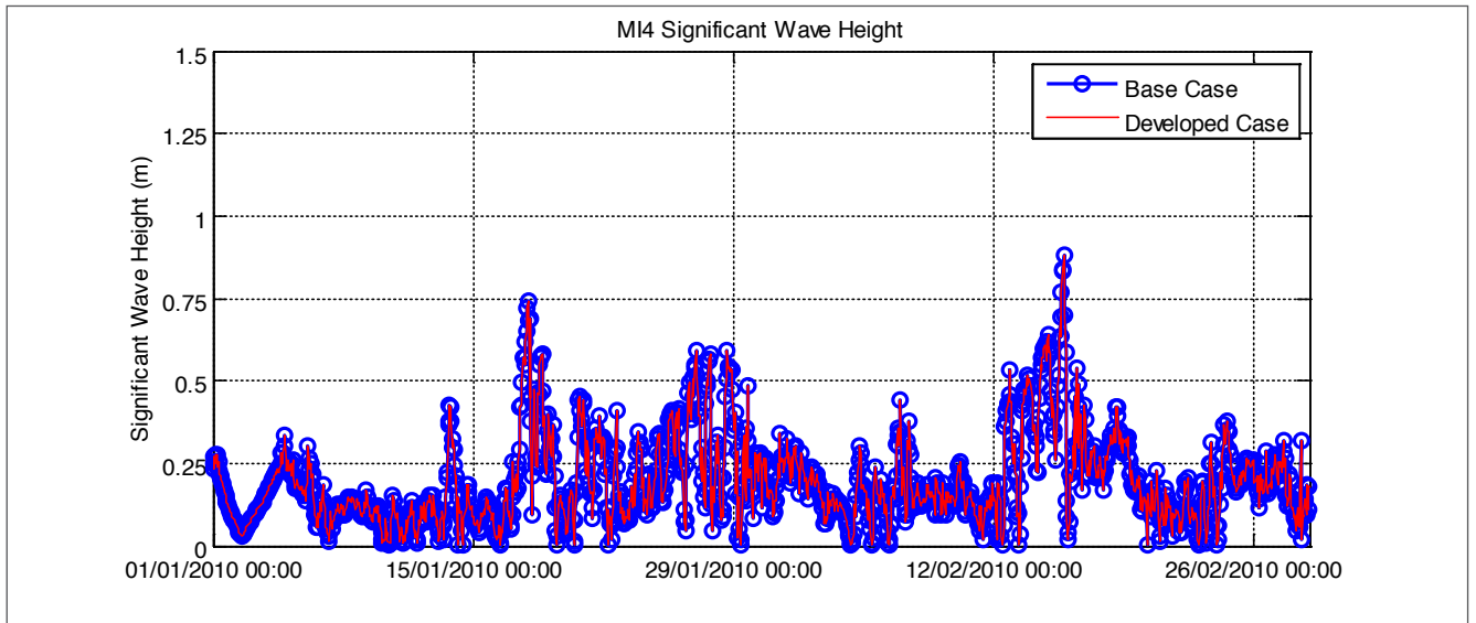
Figure B6: Wave impacts at the shoreline – location M14
