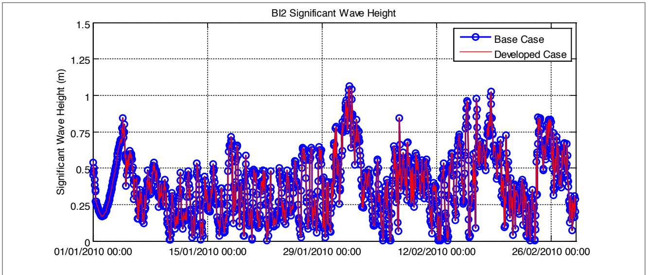
Figure B2: Wave impacts at the shoreline – location B2
