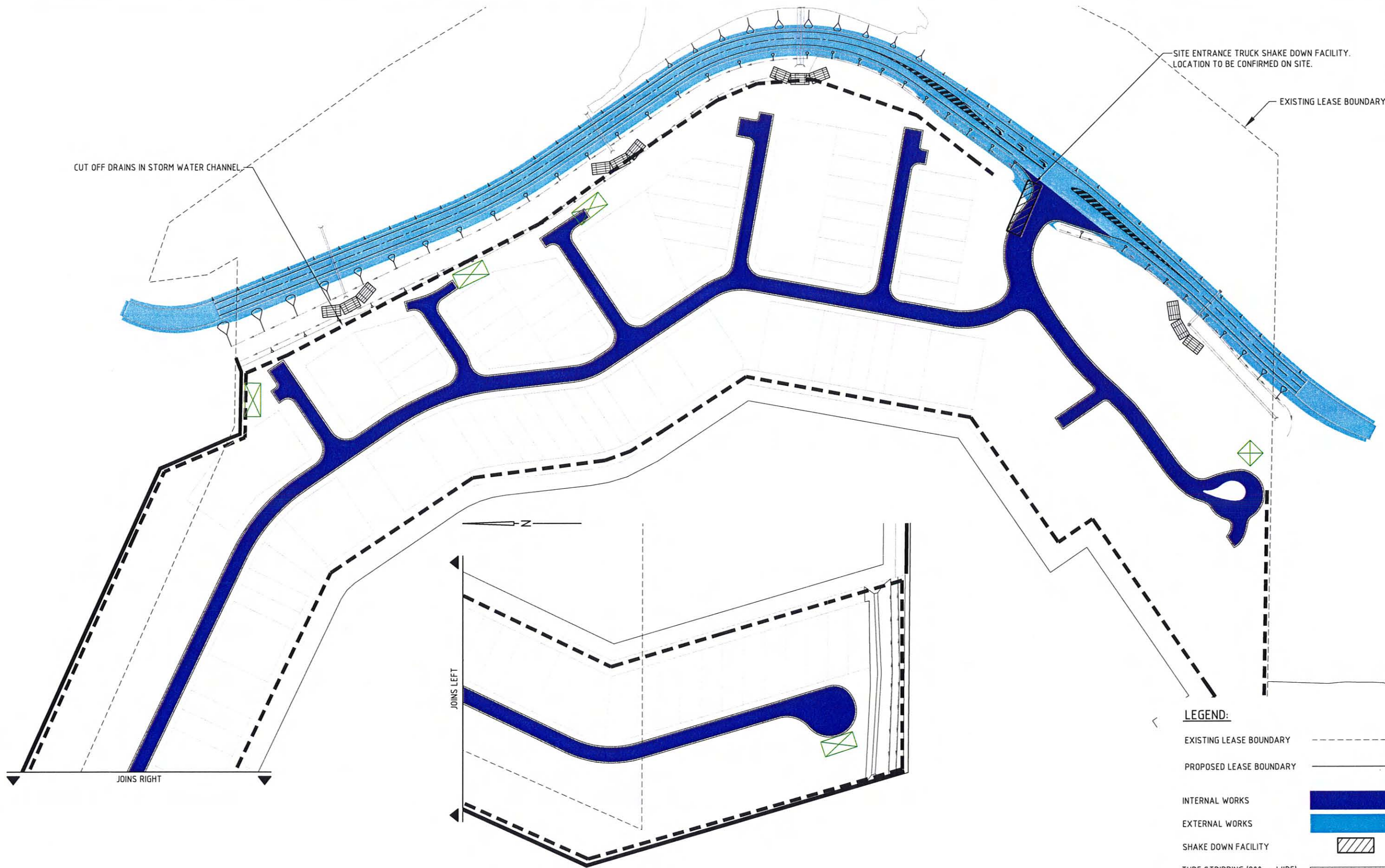
PHASE 5 PLAN SCALE 1:1000
