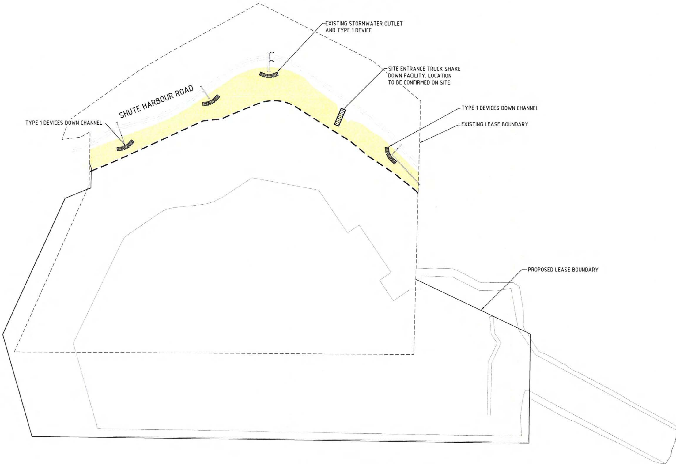
PHASE 1 PLAN SCALE 1:2000
