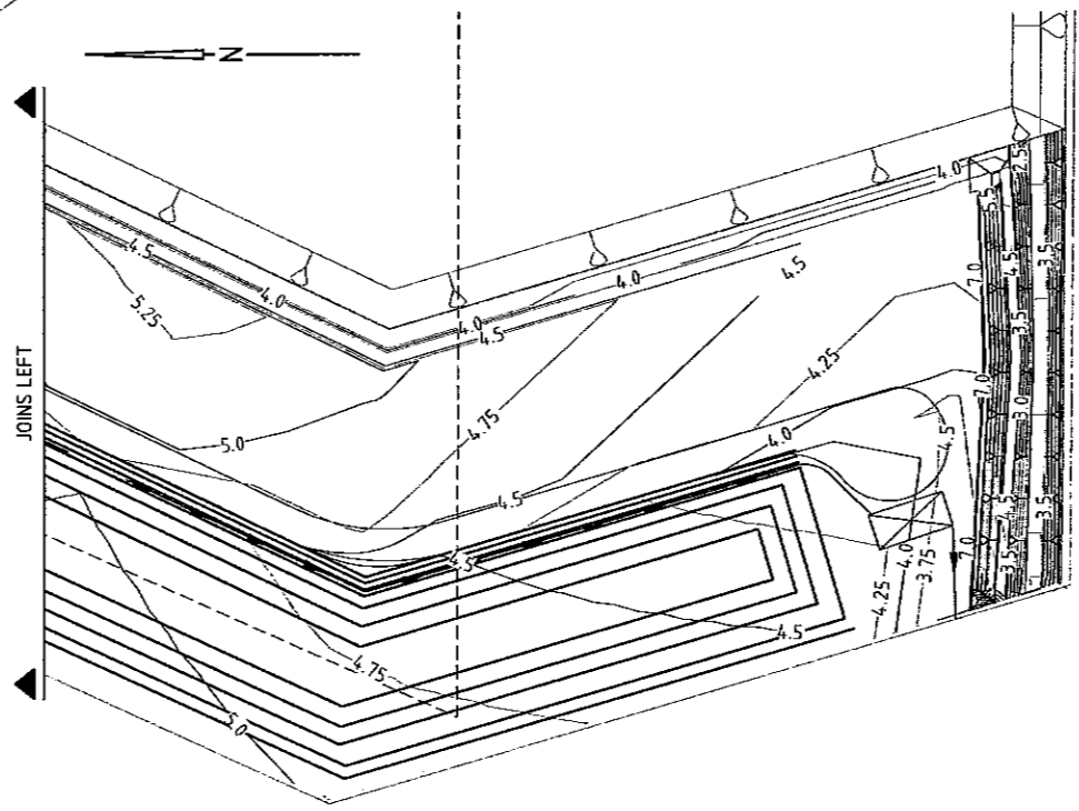
LAYOUT PLAN SCALE 1:1000
