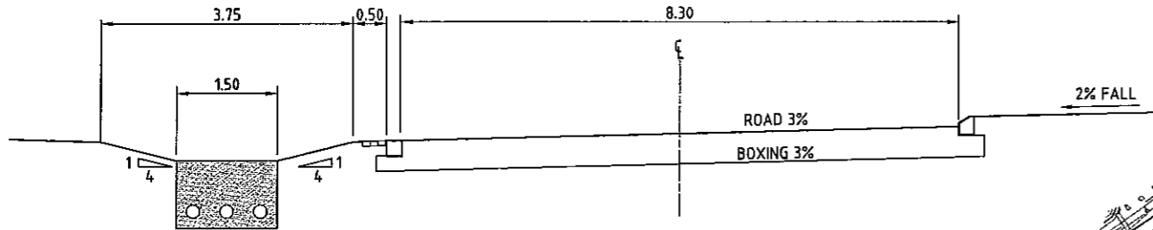
SECTION 1 SCALE 1:50
