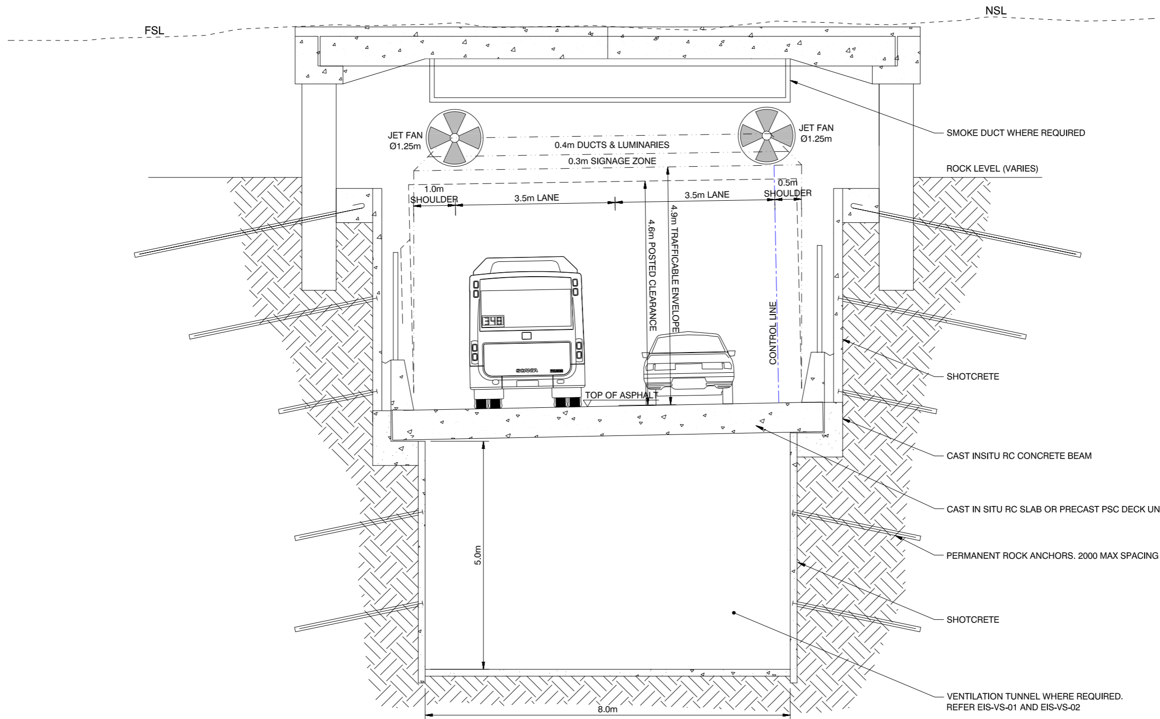
CUT AND COVER WITH VENTILATION TUNNEL
