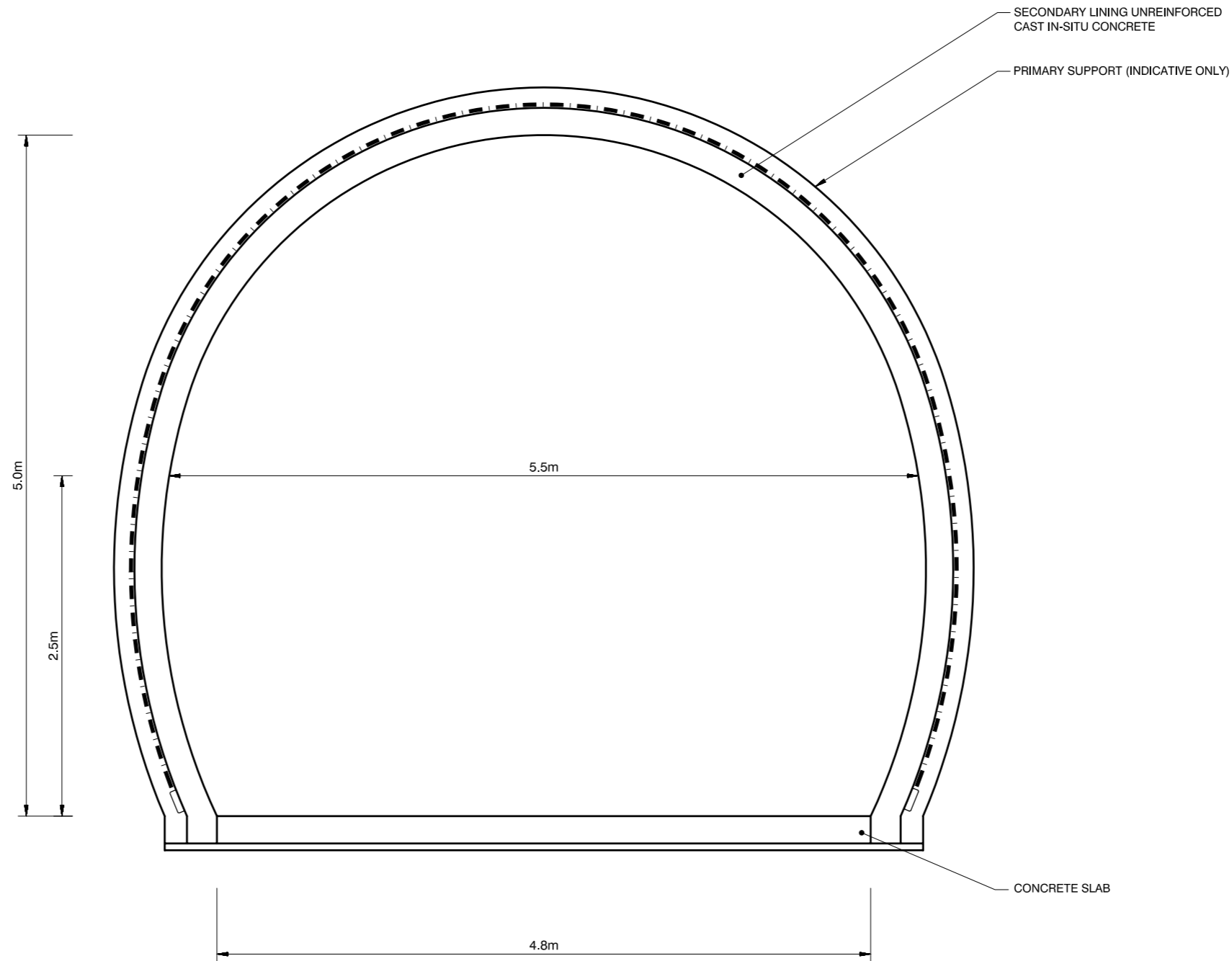
TYPICAL CROSS PASSAGE
