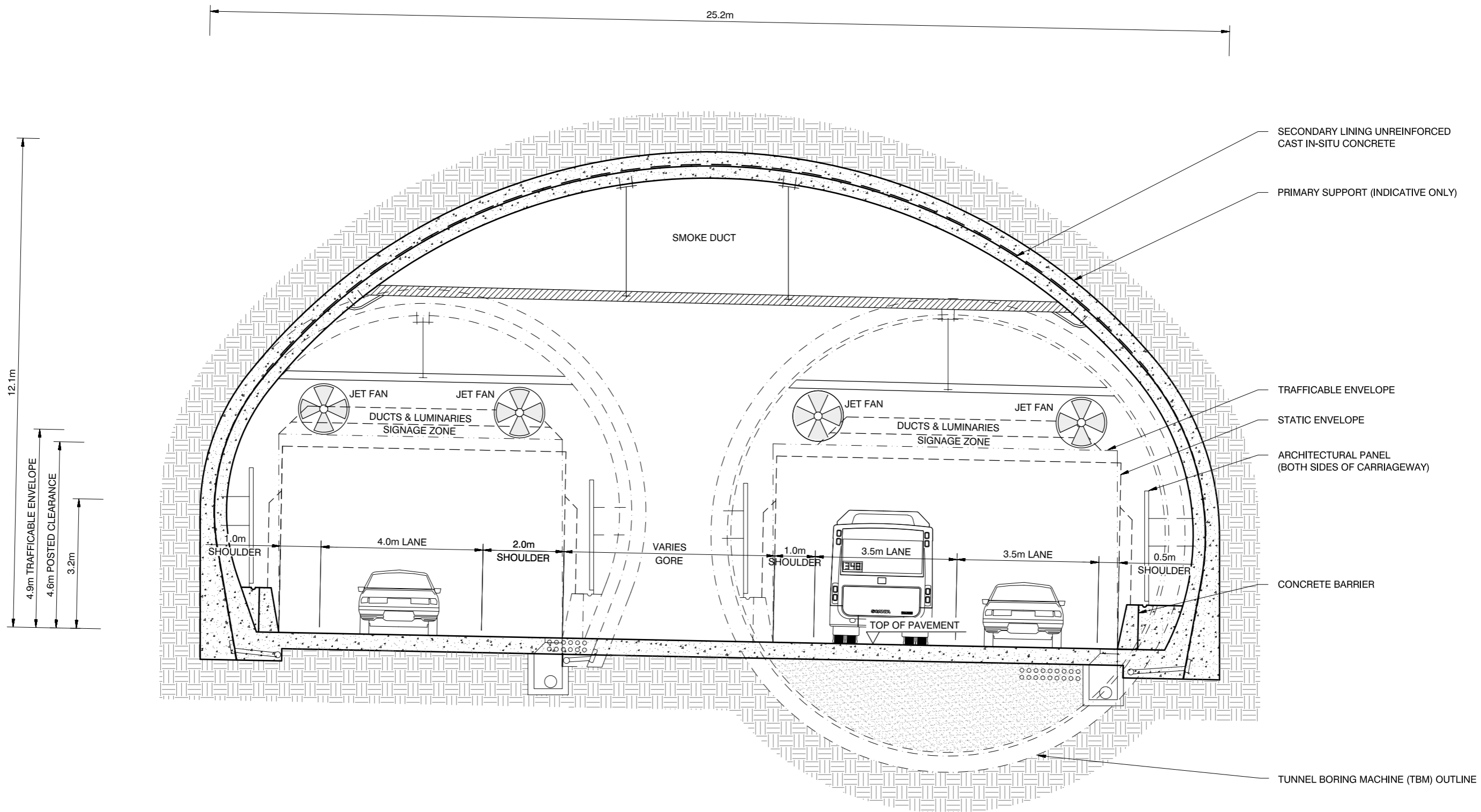
THREE LANE ROADHEADER TUNNEL AT Y-JUNCTION
