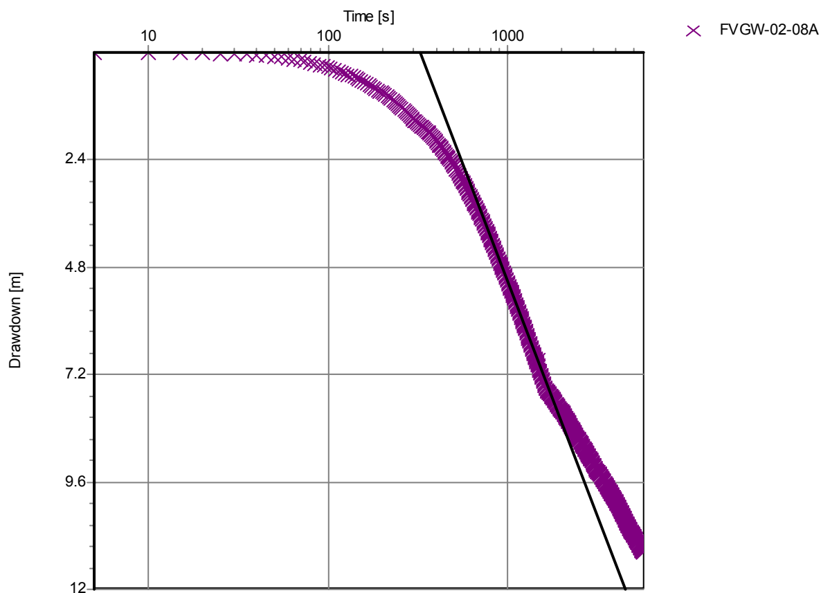
FVGW-02-08A [Cooper-Jacob Time-Draw down]
