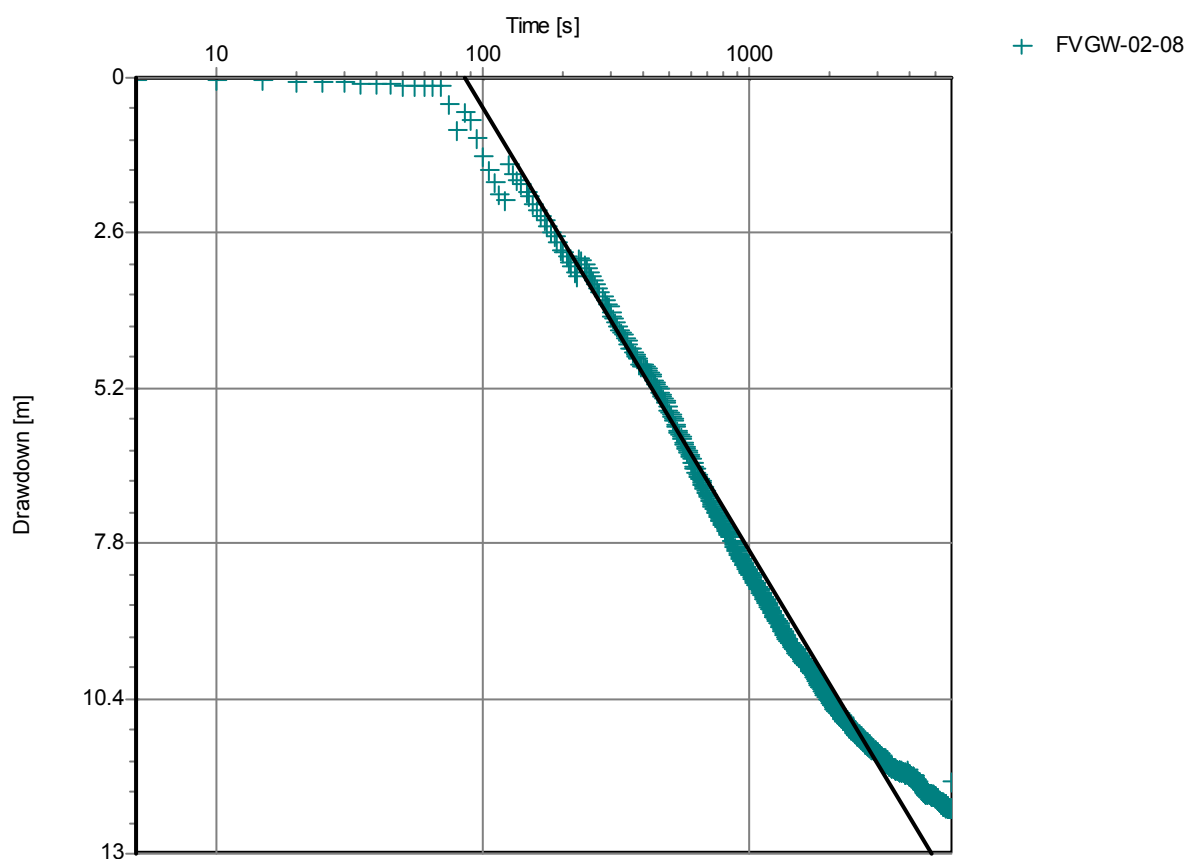
FVGW-02-08 [Cooper-Jacob Time-Draw down]
