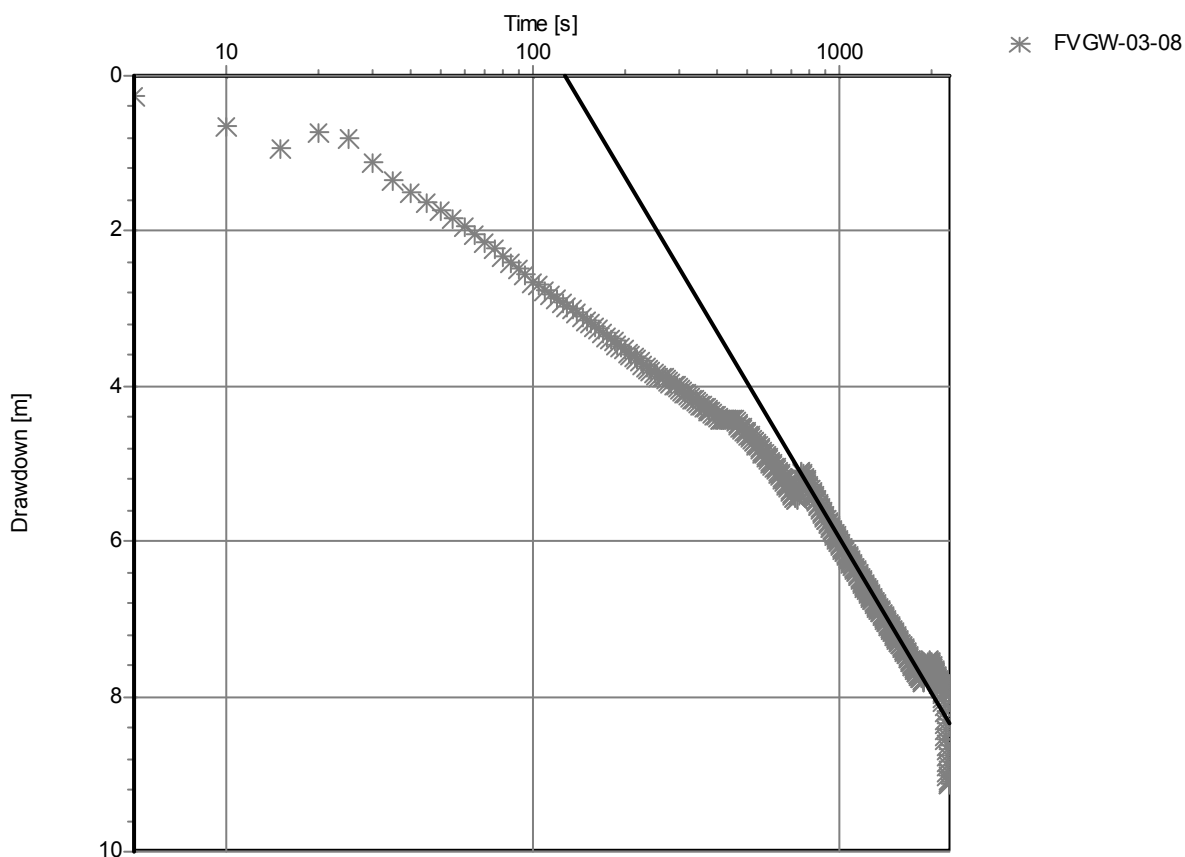
FVGW-03-08 [Cooper-Jacob Time-Draw down]
