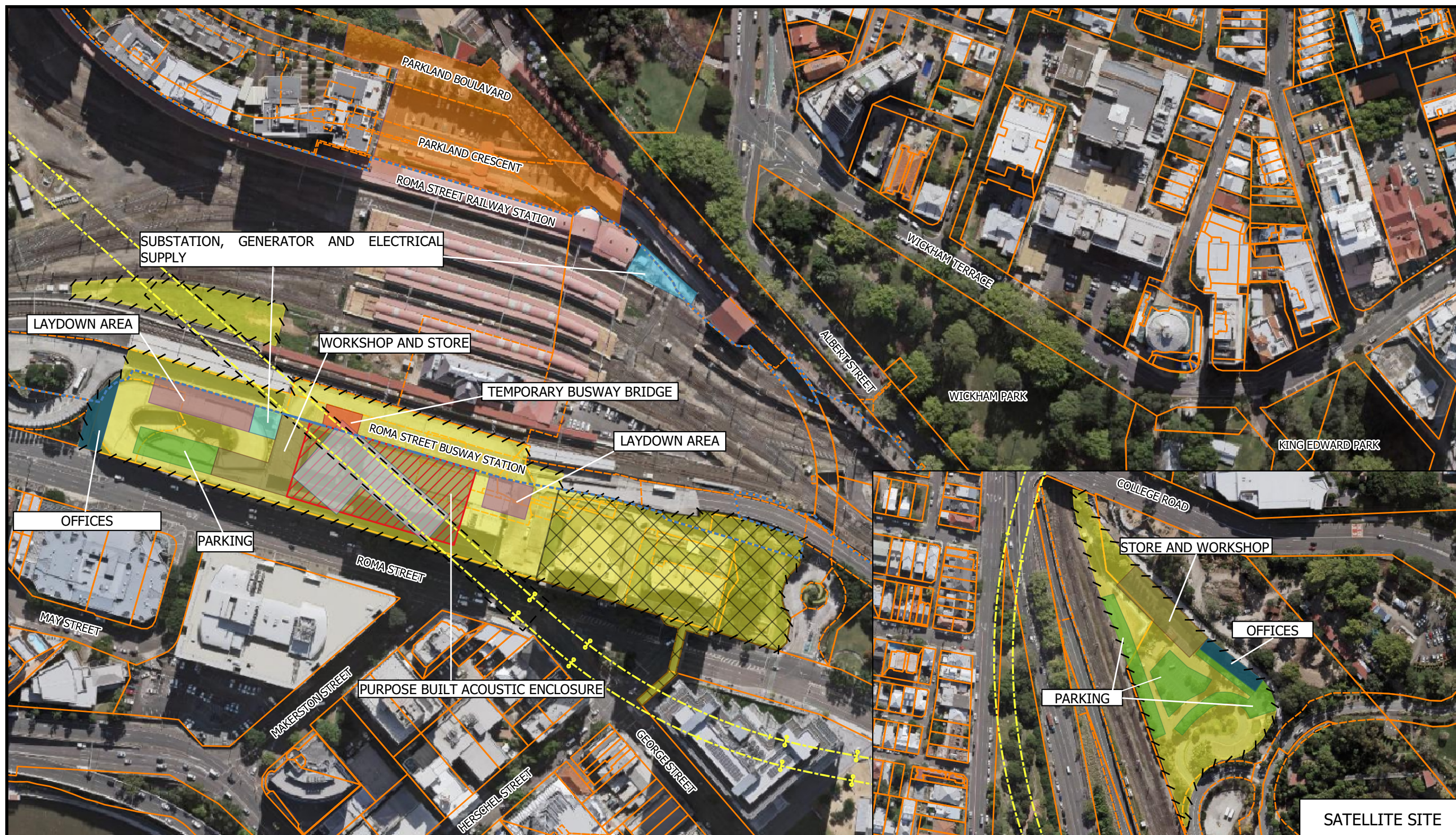
Figure 5: Changed Construction Site Plan
