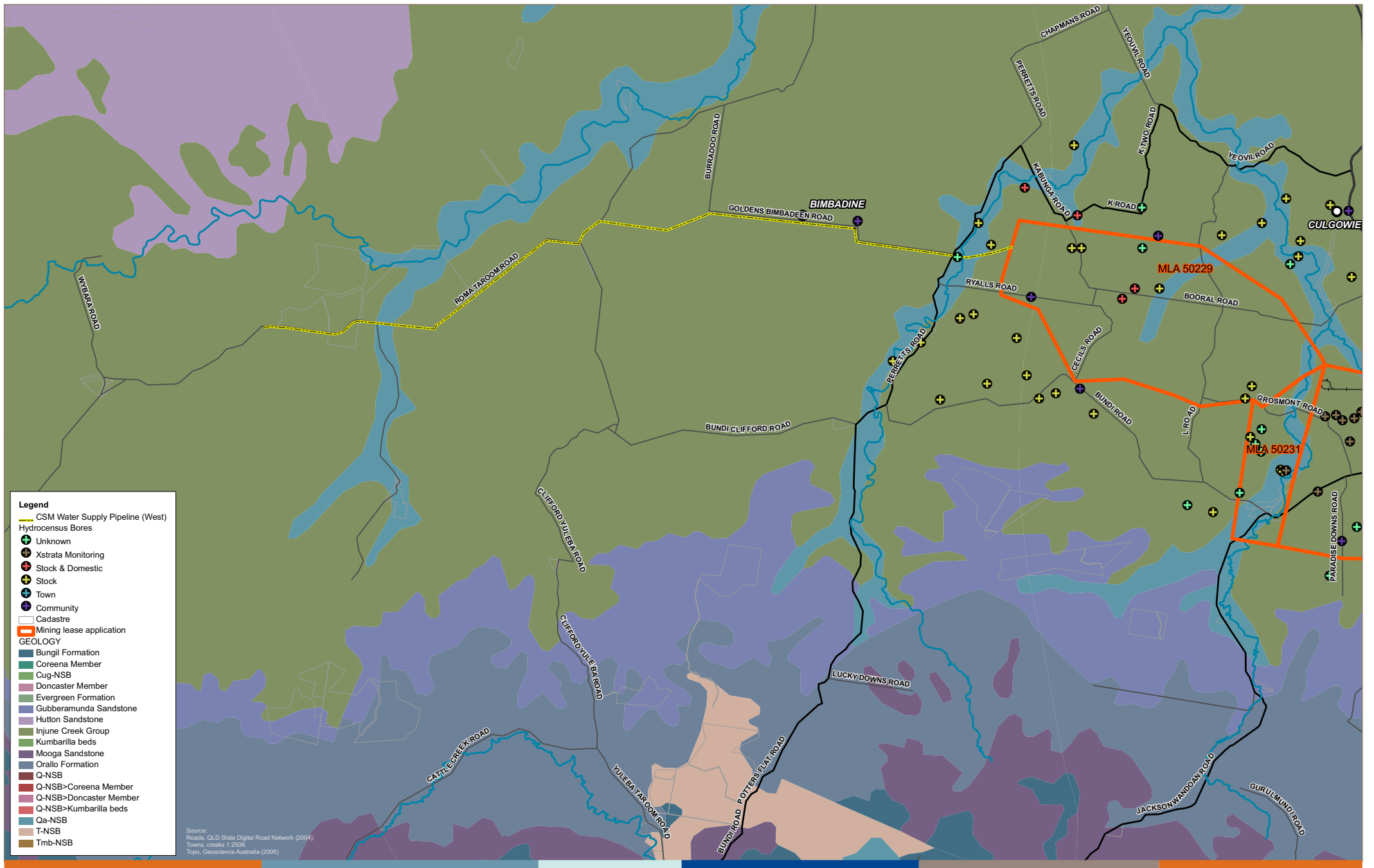
Figure 10-2-V3.3 Geology of the Western Pipeline Area
