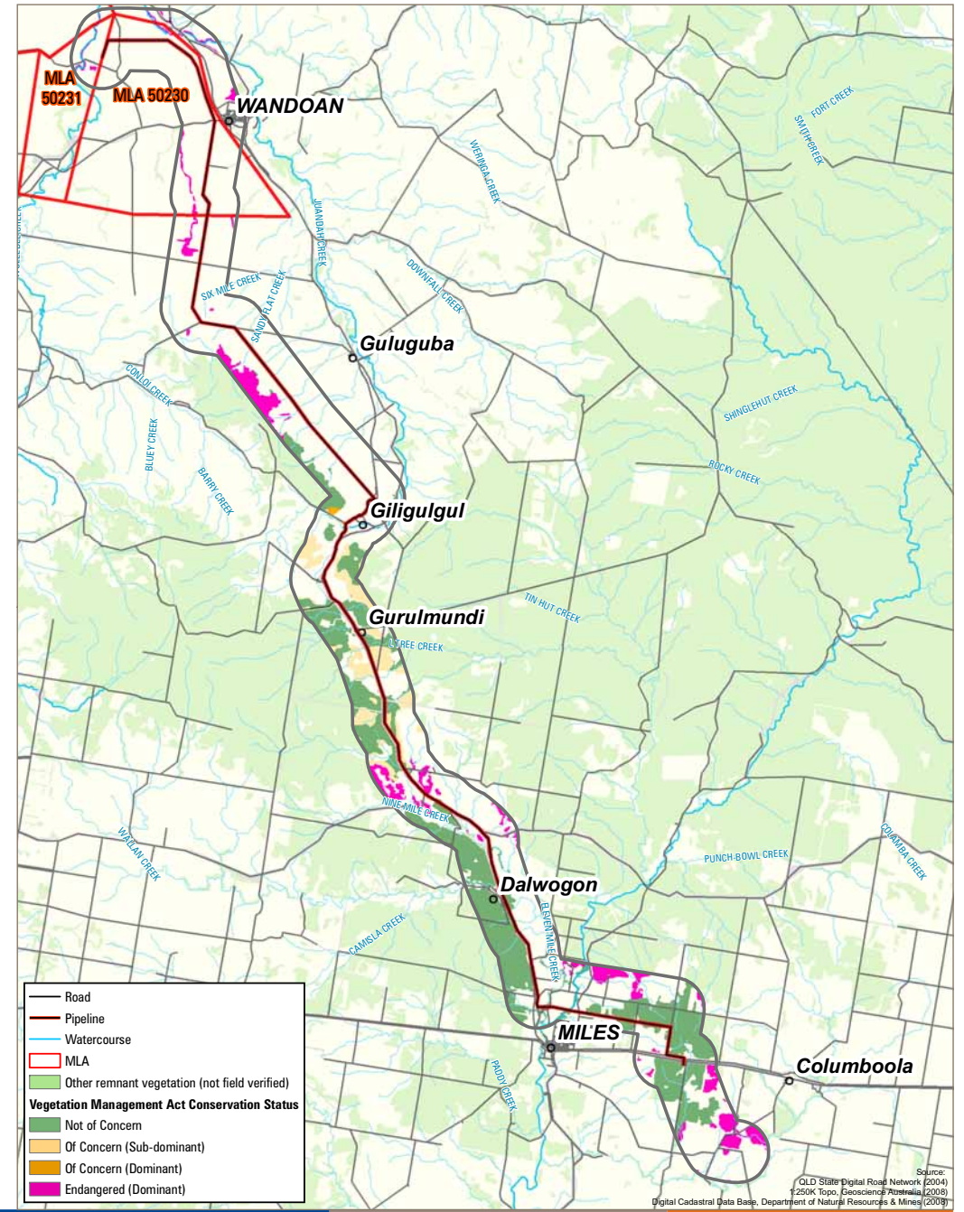
Figure 17A-2-V2.3 Regional ecosystems within the study area
