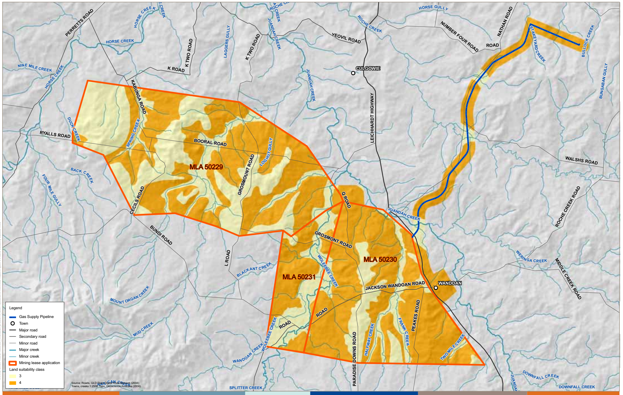
Figure 9-9-V1.3 Land suitability for rainfed cropping
