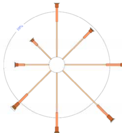
Figure 7-4: Wind Rose, Northern extent 3pm
