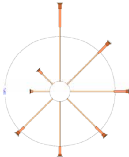
Figure 7-1: Wind Rose, Southern extent 9am
