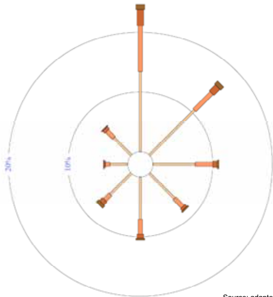
Figure 7-1: Wind Rose, Southern extent 9am
