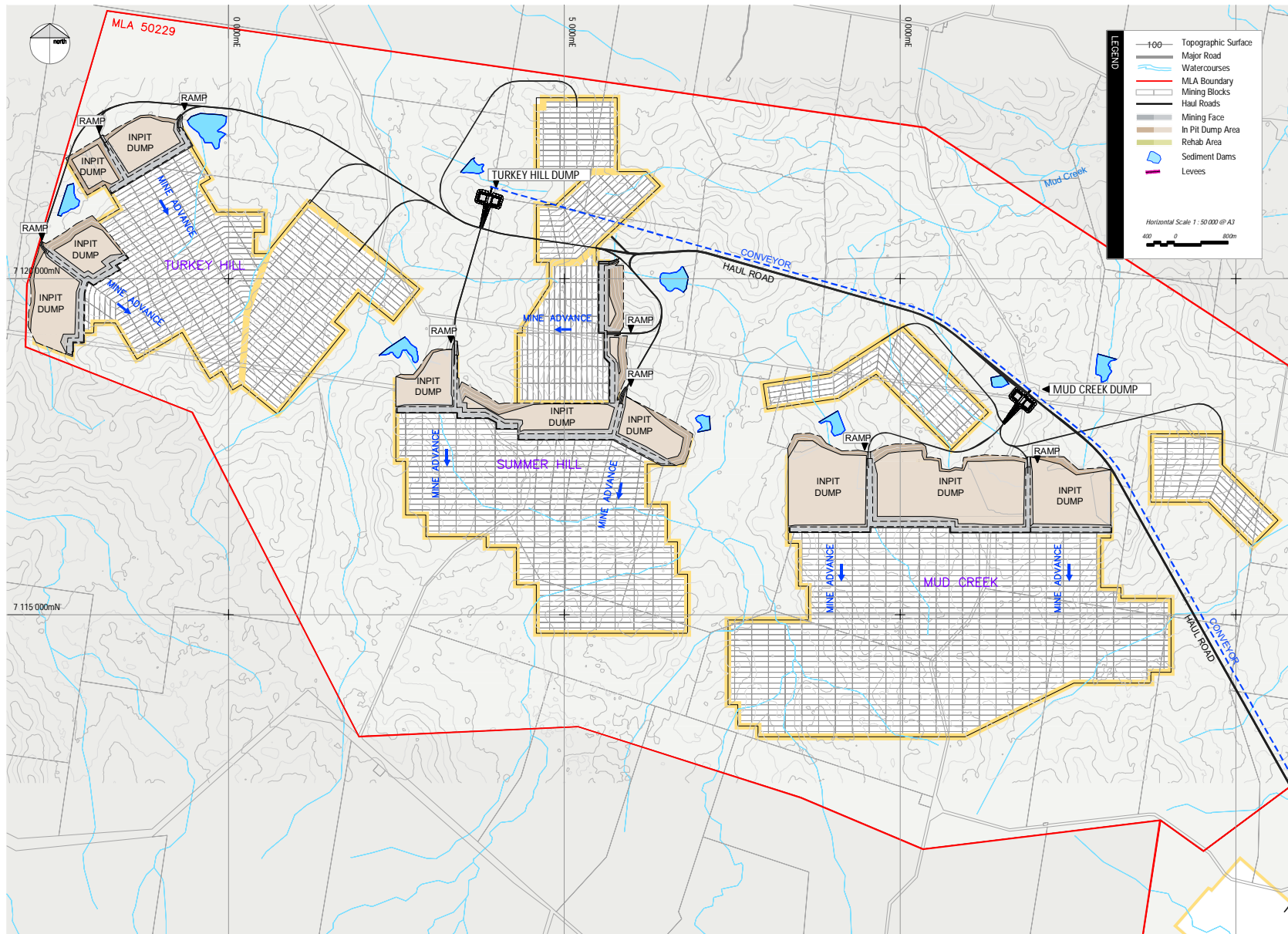
Figure 6-9-V1.3 Year 10 Excavation & Refill Plan for MLA 50229
