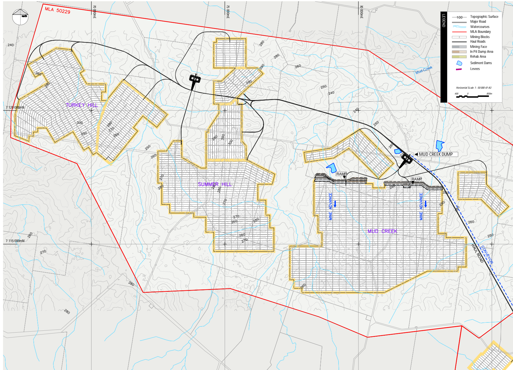
Figure 6-7-V1.3 Year 5 Excavation & Refill Plan for MLA 50229
