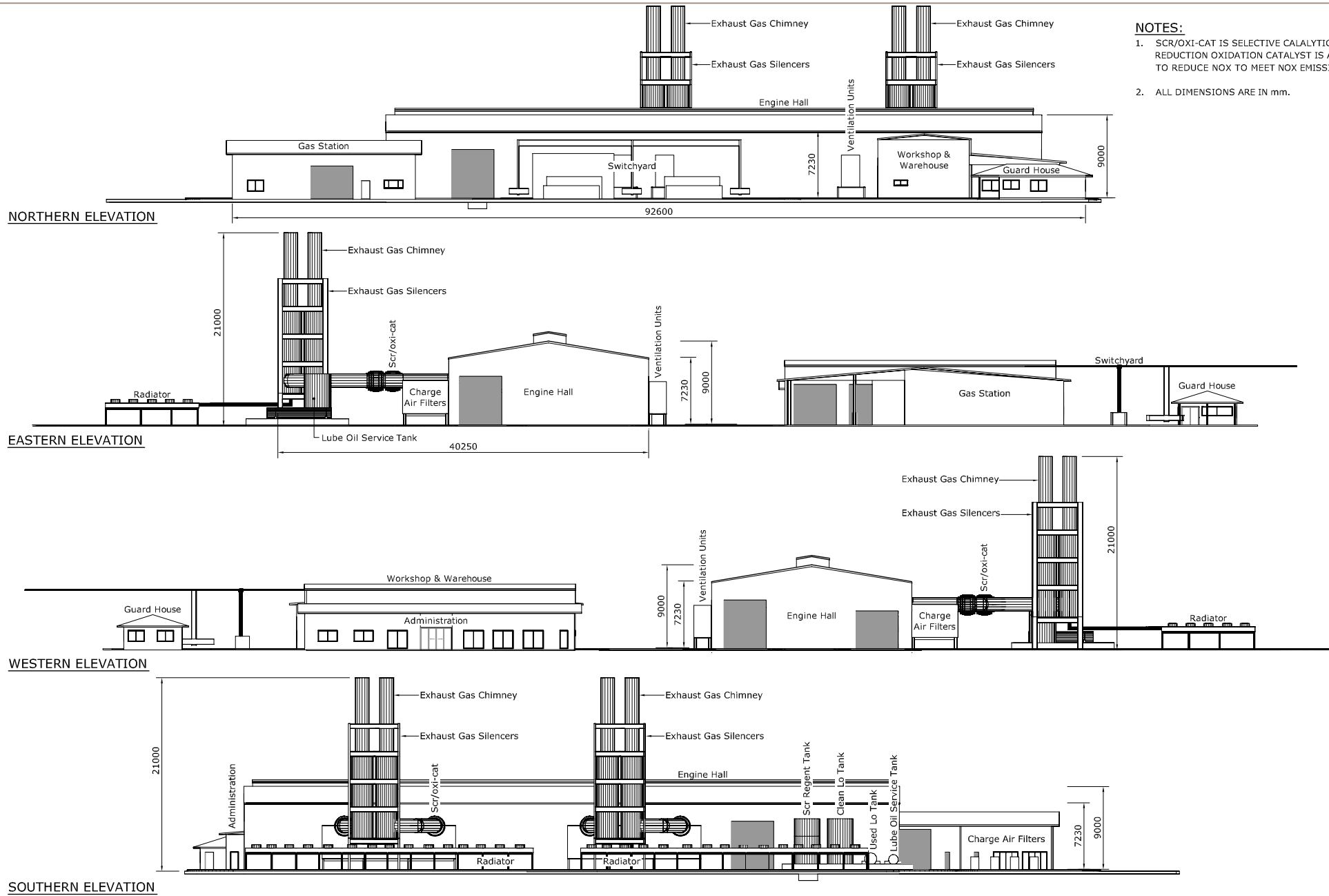
Figure 6-40-V1.3 Indicative Elevation - 30MW Gas-fired Power Station Option
