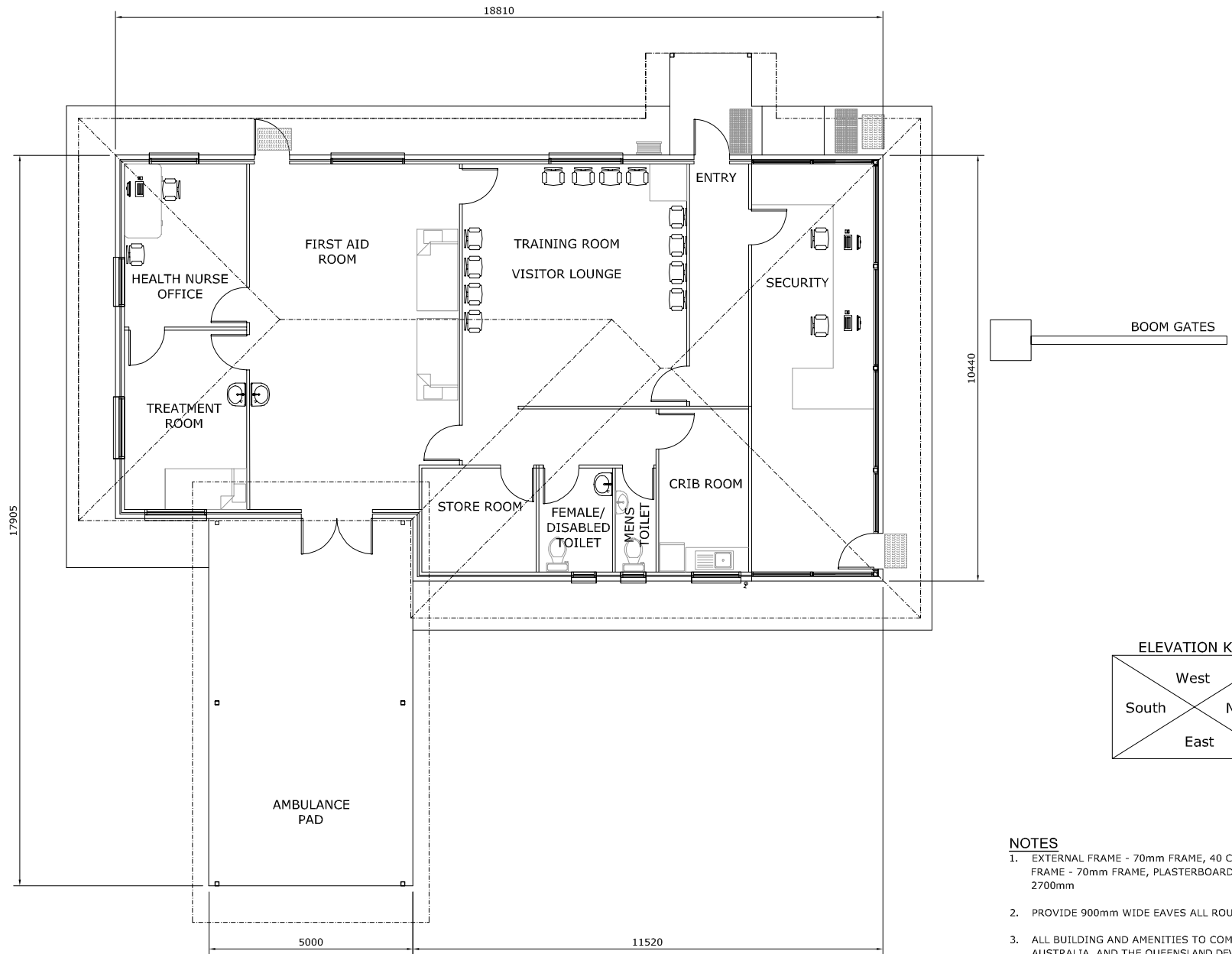
Figure 6-33-V1.3 Indicative Layout - Main Gate & Security Building
