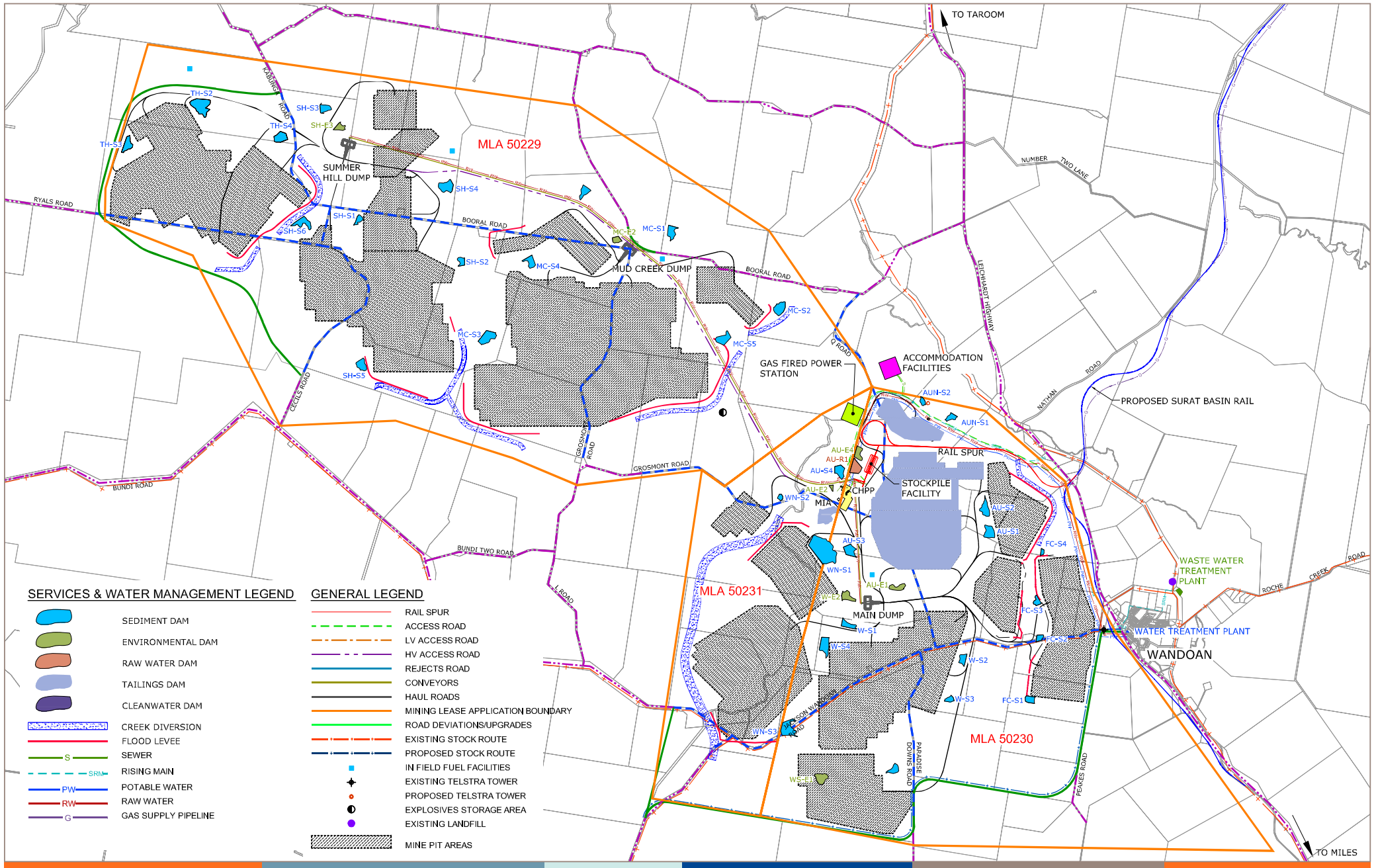
Figure 6-30-V1.3 Indicative Operational Mine Facilities - Year 30
