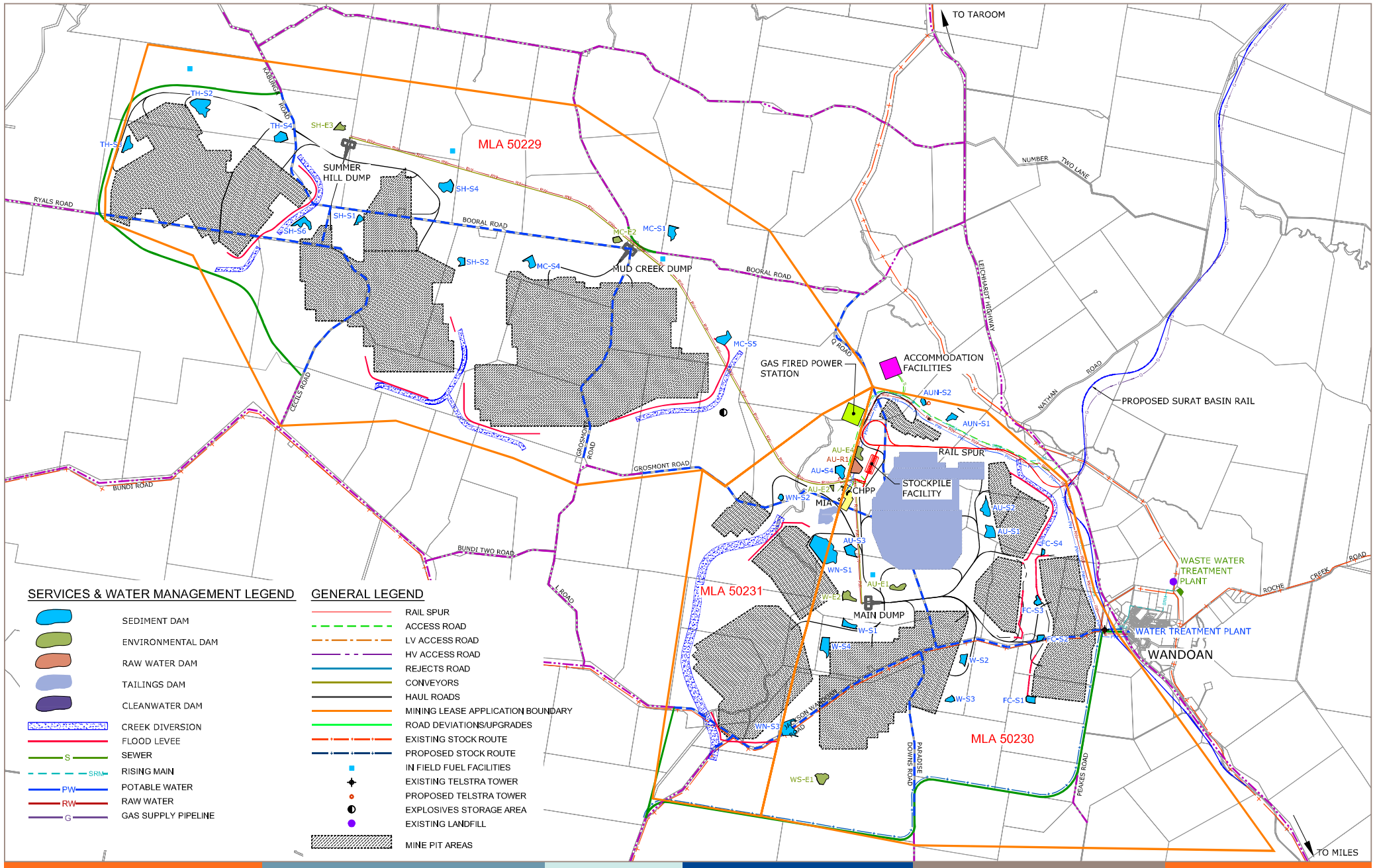
Figure 6-29-V1.3 Indicative Operational Mine Facilities - Year 20
