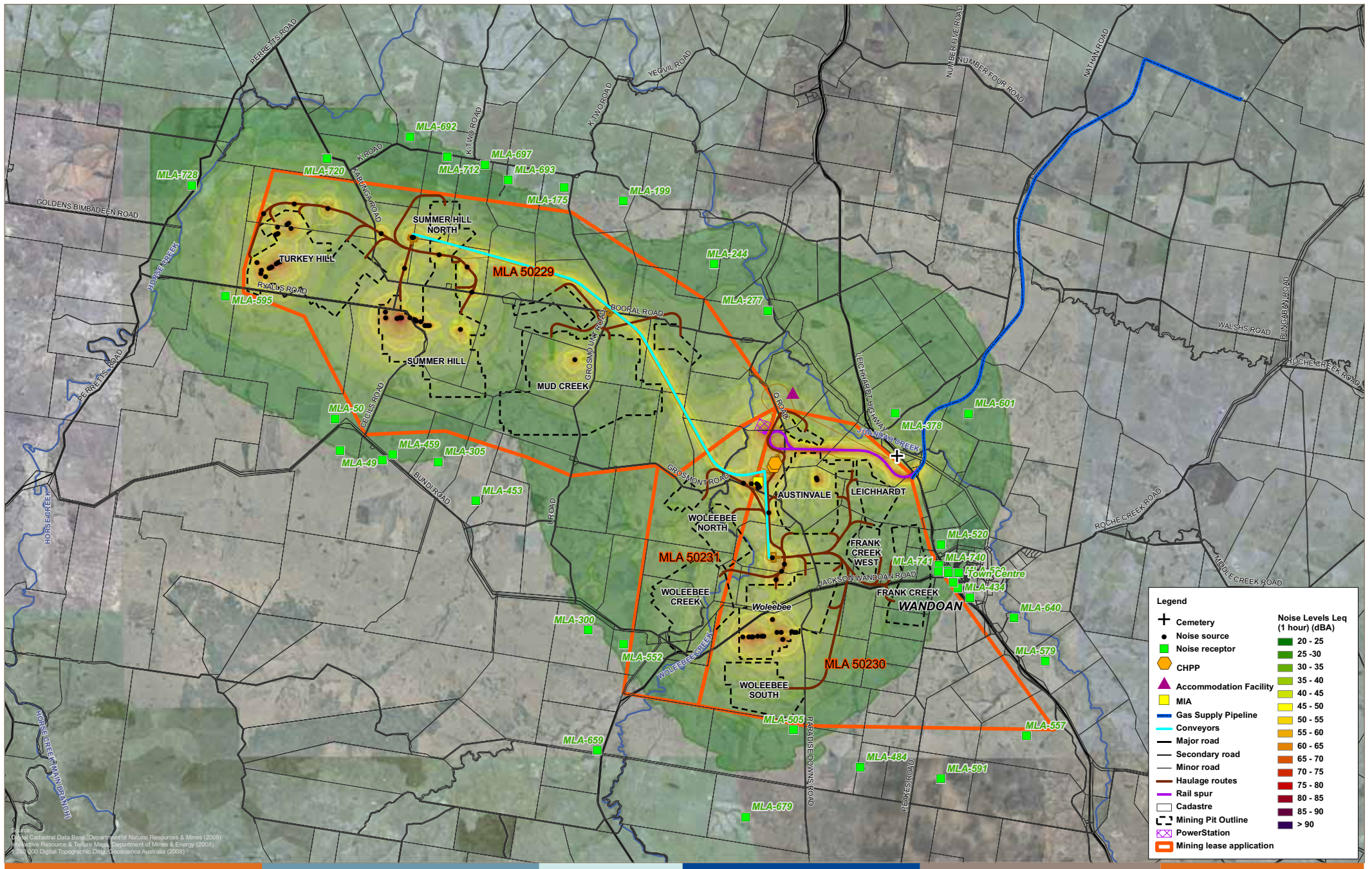
Figure 15-6-V1.3 Noise contours Scenario 4 attenuated equipment
