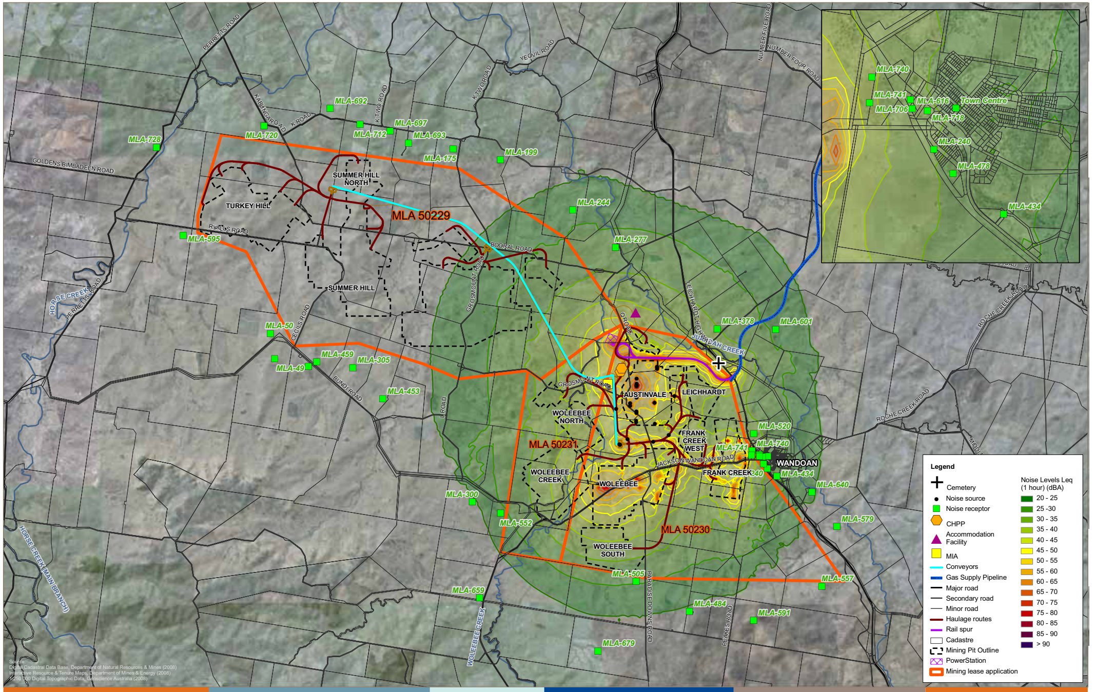
Figure 15-5-V1-3 Noise contours Scenario 3c/d attenuated dragline bucket
