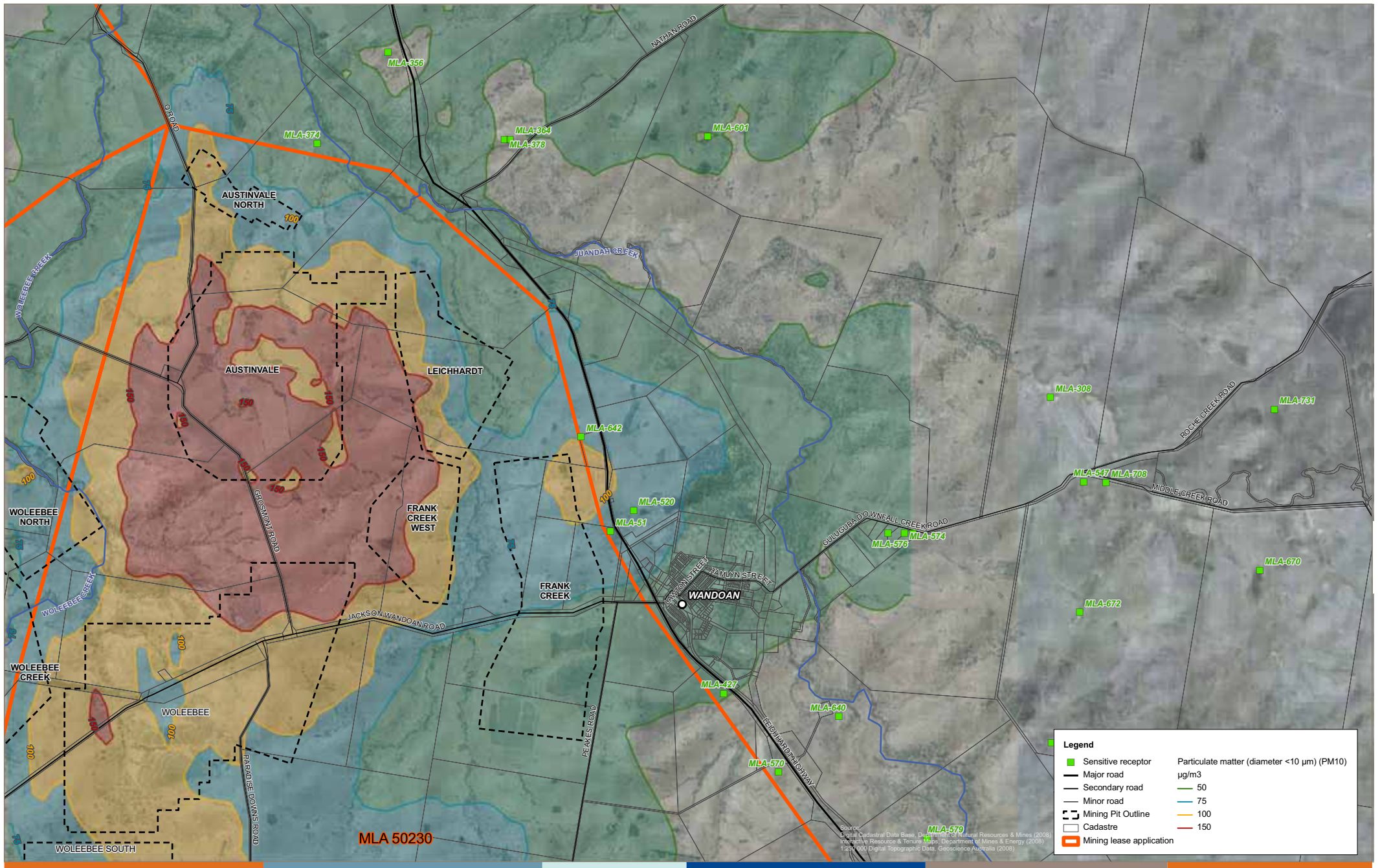
Figure 13-6-V1.3 Year 1, PM10 maximum 24 hour ground level concentrations for the mine including background
