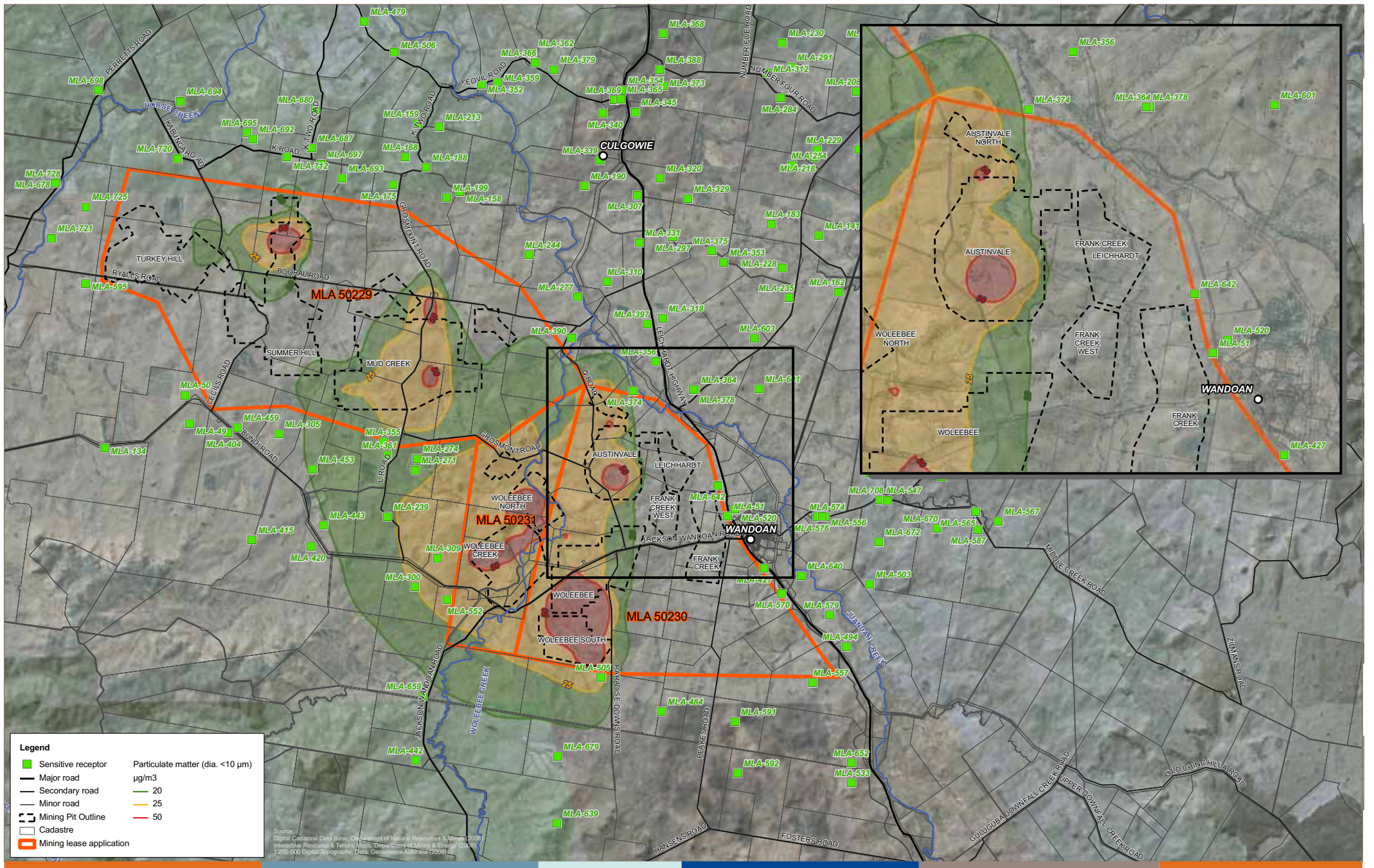
Figure 13-23-V1.3 Year 30, PM10 annual average ground level concentrations for the mine including background
