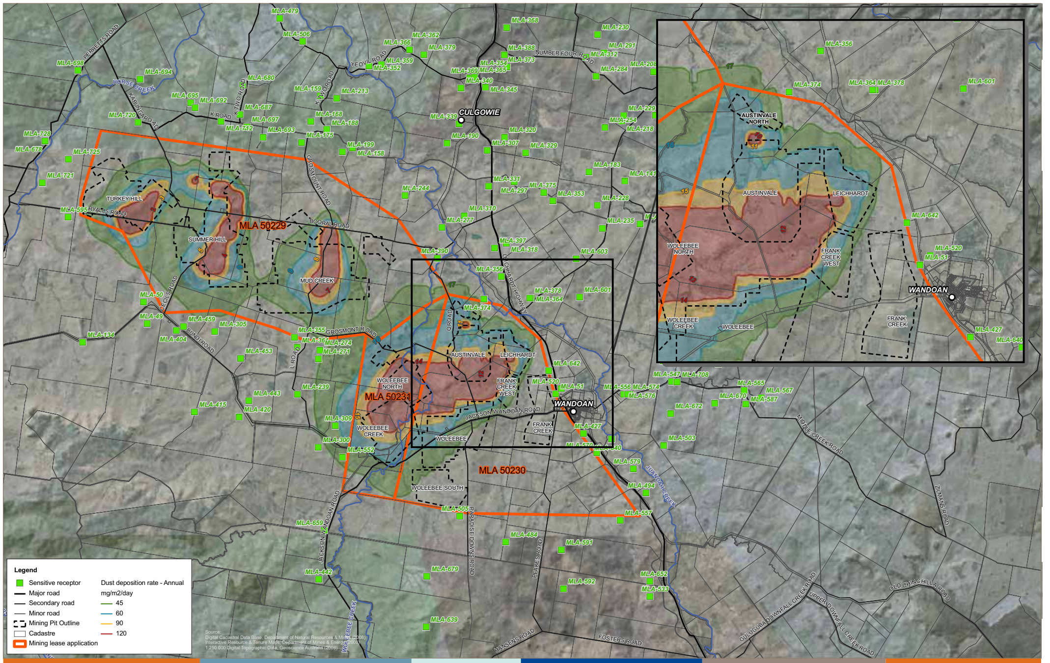
Figure 13-21-V1.3 Year 20, dust deposition for the mine including background
