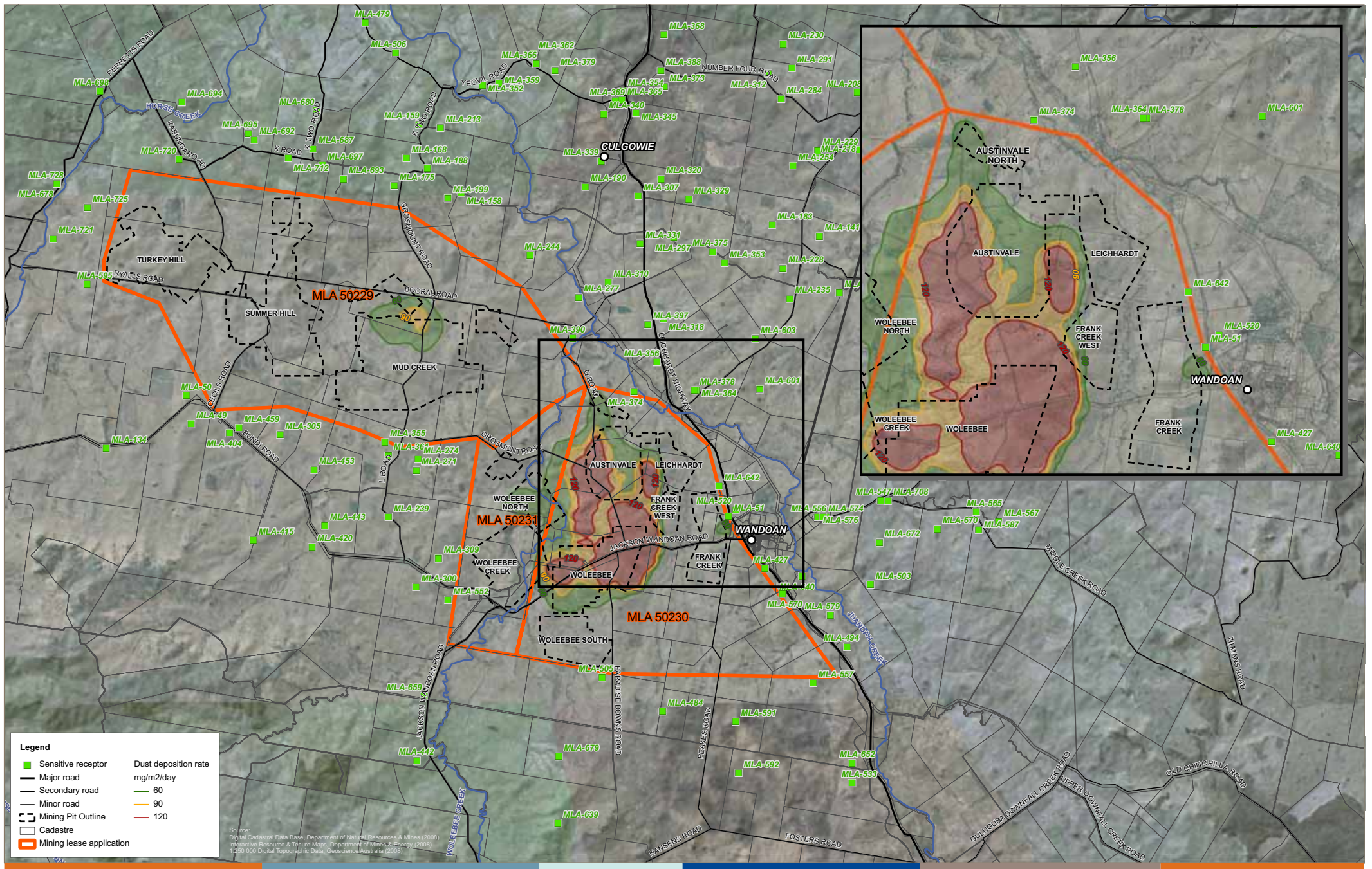
Figure 13-13-V1.3 Year 5, dust deposition for the mine including background - truck and excavator at reduced extraction rates.
