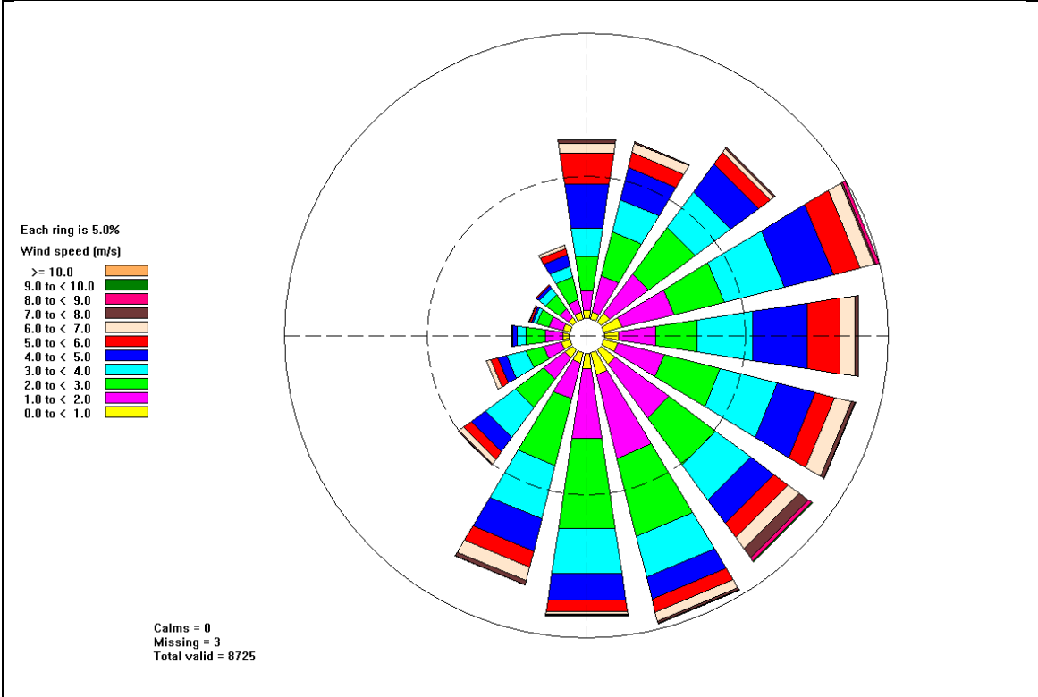
Figure 1 Wind rose for all hours at Wandoan
