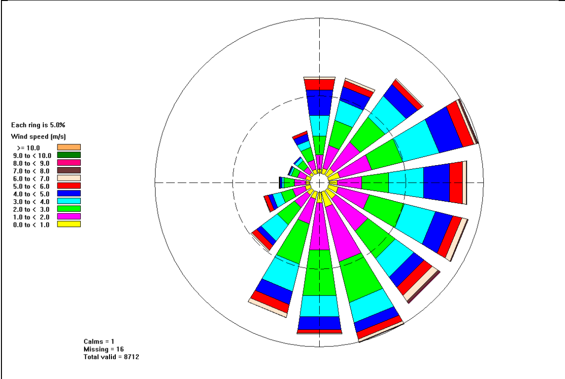
Figure 7 Wind rose for all hours for the Wandoan CALMET meteorological file
