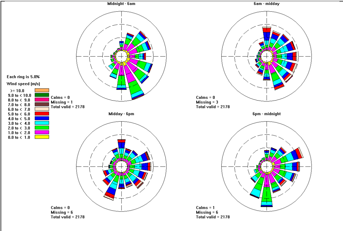
Figure 8 Wind rose according to time of day for the Wandoan CALMET meteorological file
