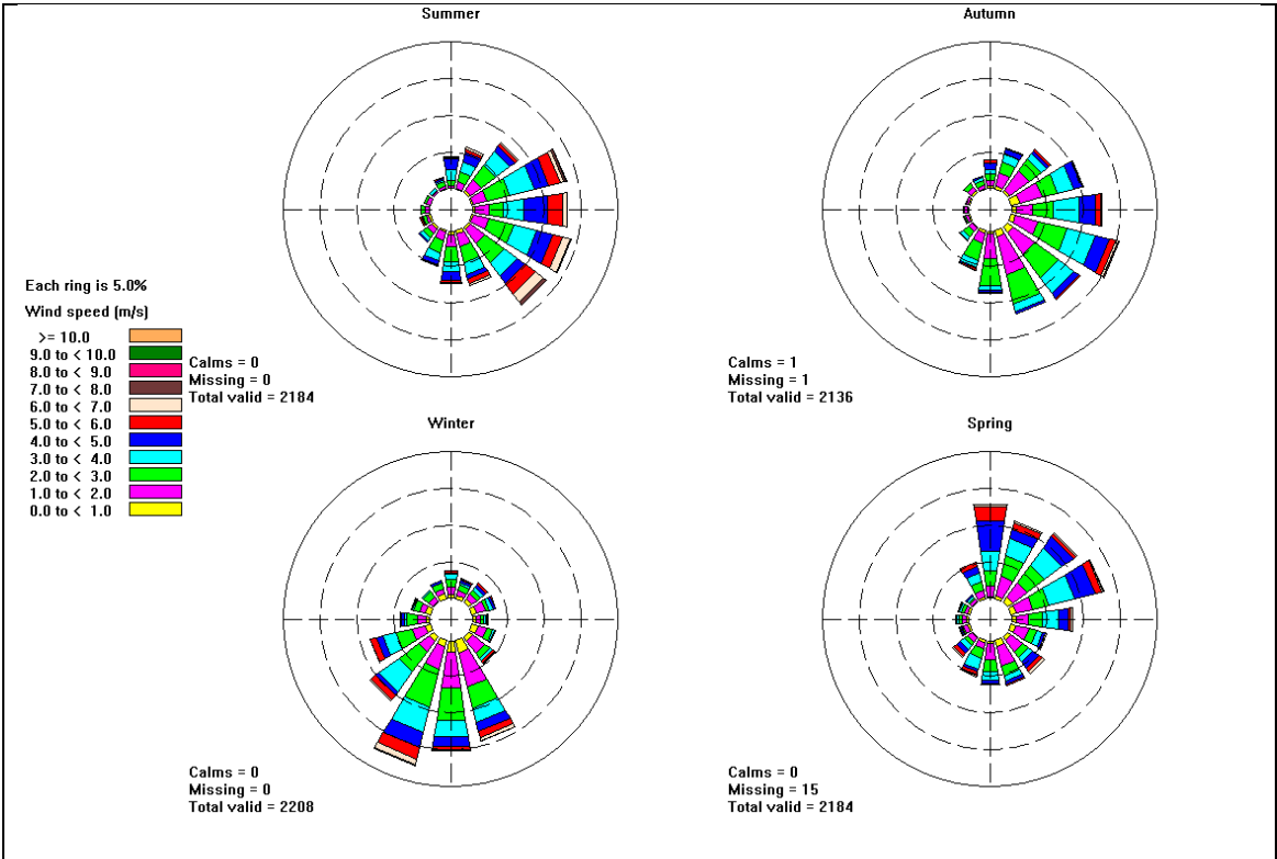
Figure 9 Seasonal wind rose for the Wandoan CALMET meteorological file
