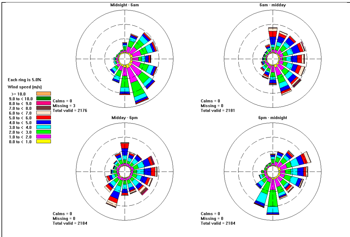
Figure 2 Wind rose according to time of day at Wandoan
