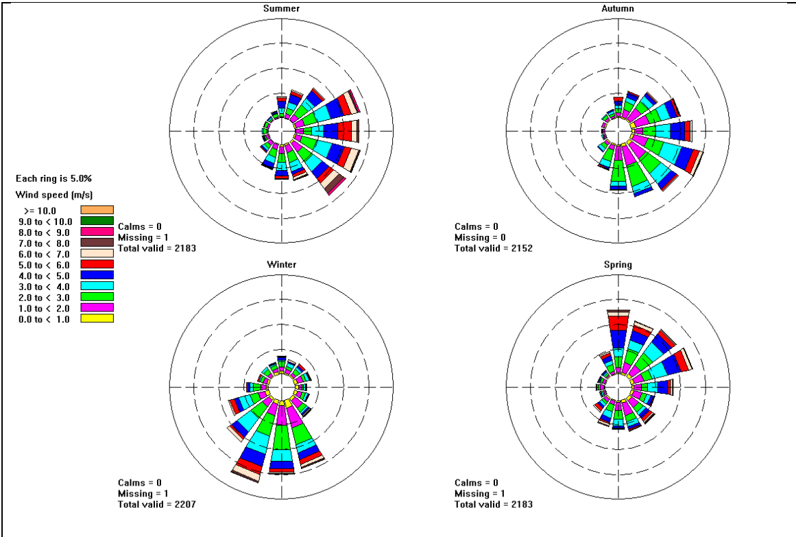
Figure 3 Seasonal wind rose at Wandoan
