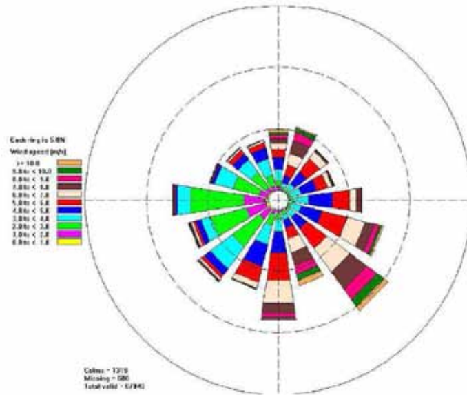
Figure 8-1 Annual Wind Rose
