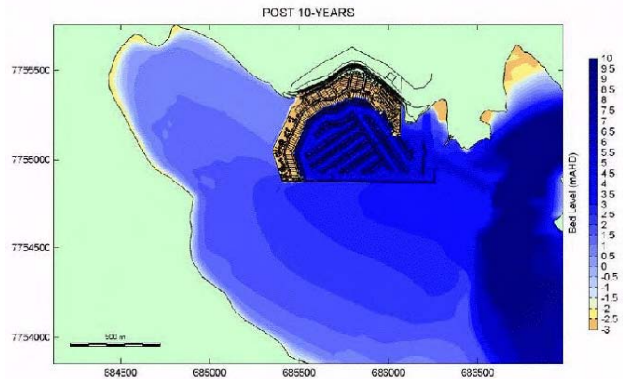
Scale NTS (A3) FIGURE 20 COASTAL SILTATION PROCESSES
