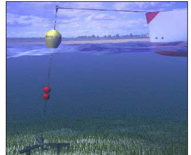
Low Impact to Seagrass Moorings Image sourced from Advanced Mooring Technologies.
