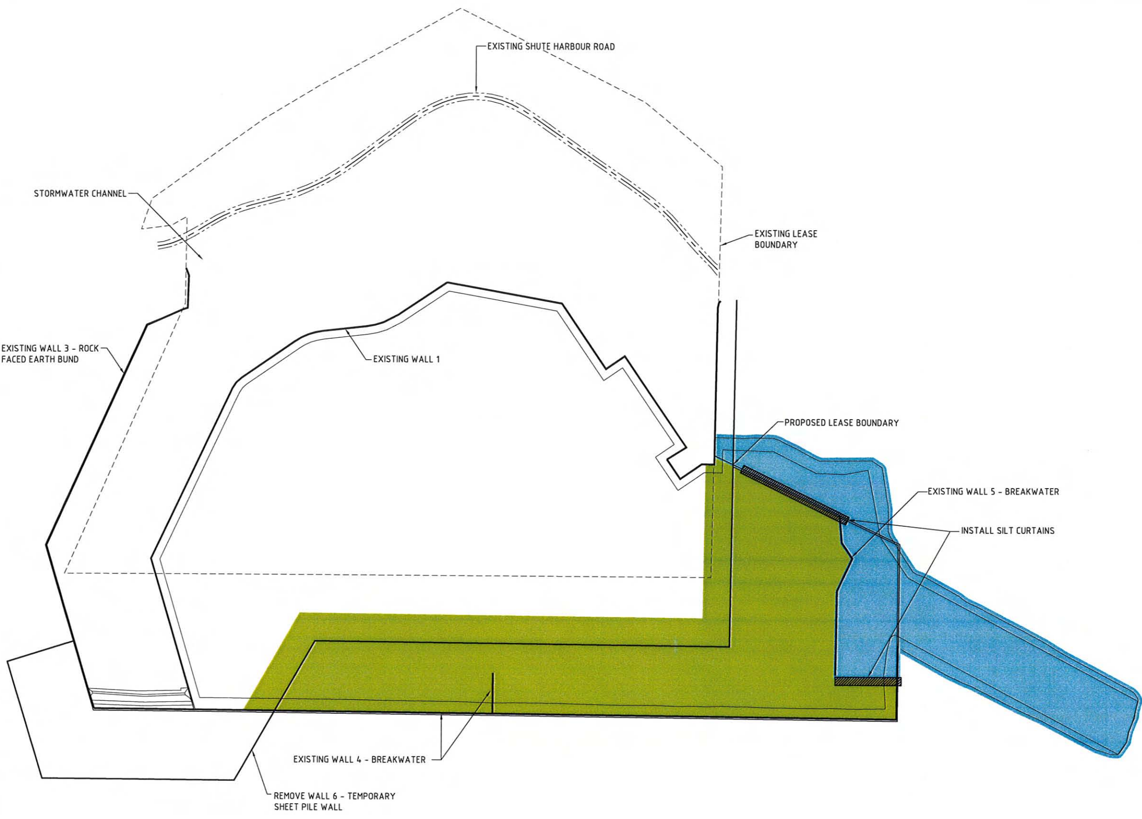
PHASE 4 PLAN SCALE 1:2000
