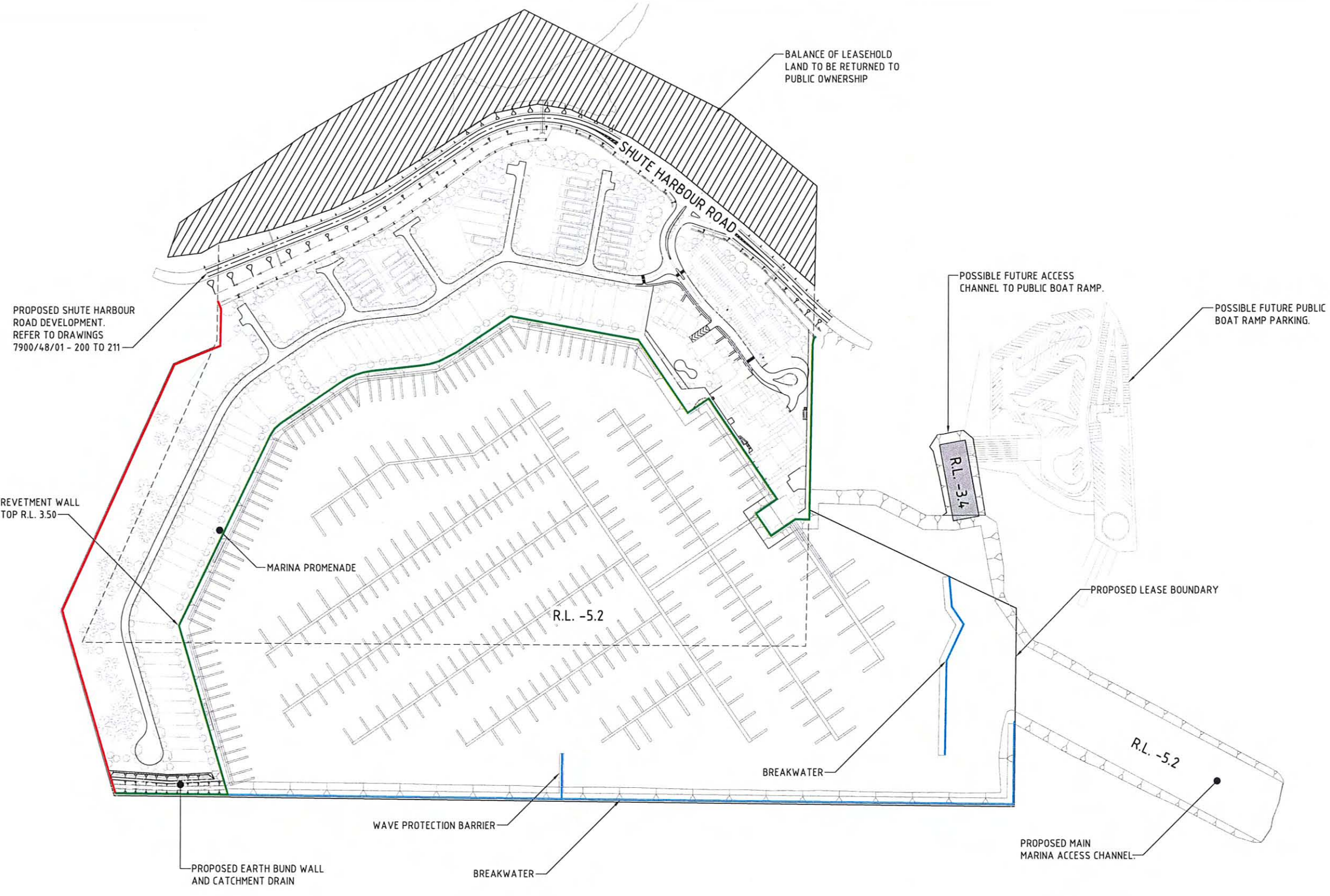
LAYOUT PLAN 1:2000
