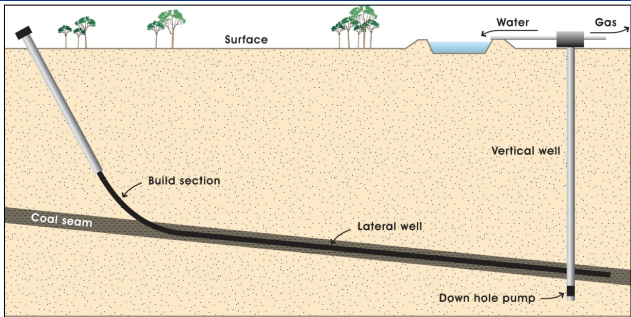
Figure 3-6 Indicative Layout of Surface to Inseam Drilling
