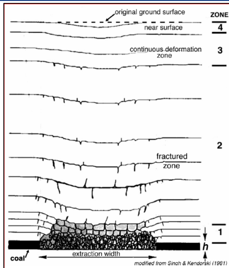
Figure 3-2 Typical Subsidence Profile (from Winters and Capo 2004)
