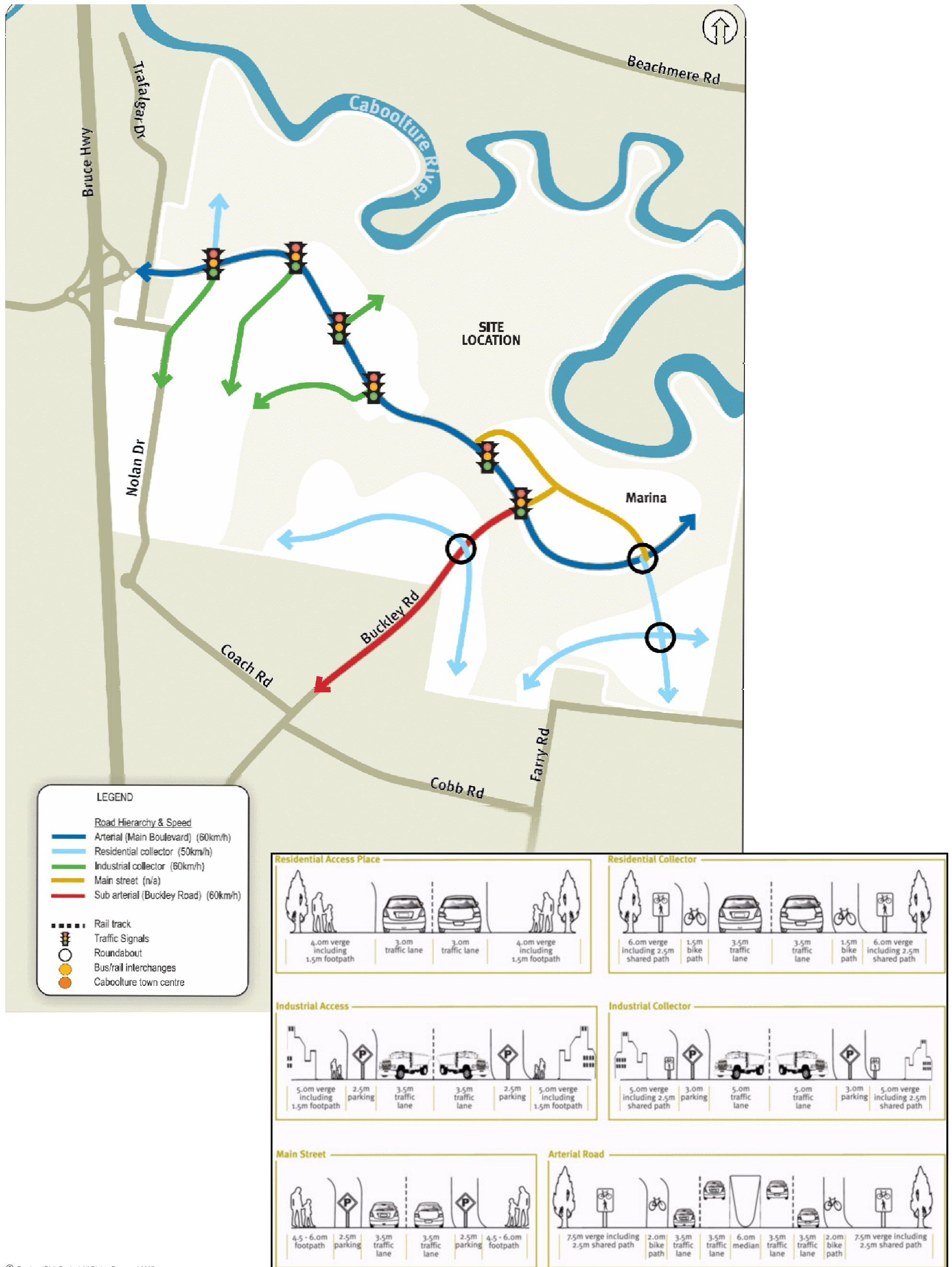
FIGURE 10 CONCEPTUAL ROAD LAYOUT AND CROSS SECTIONS
