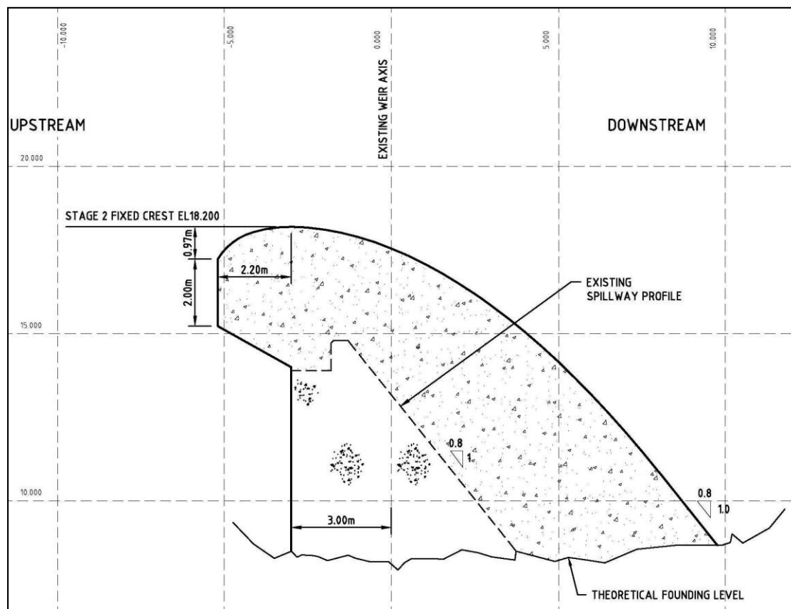
Figure 2-10 Eden Bann Weir Stage 2 ogee spillway section
