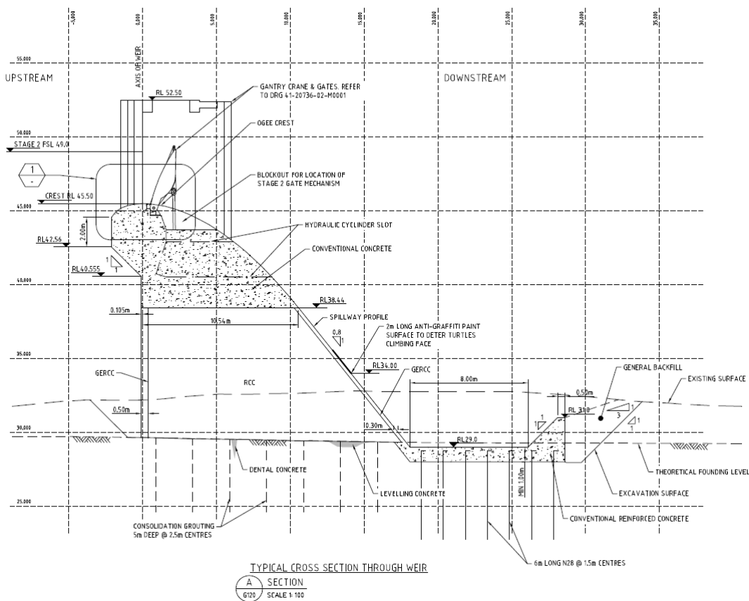
Figure 2-16 Rookwood Weir Stage 2 ogee spillway section
