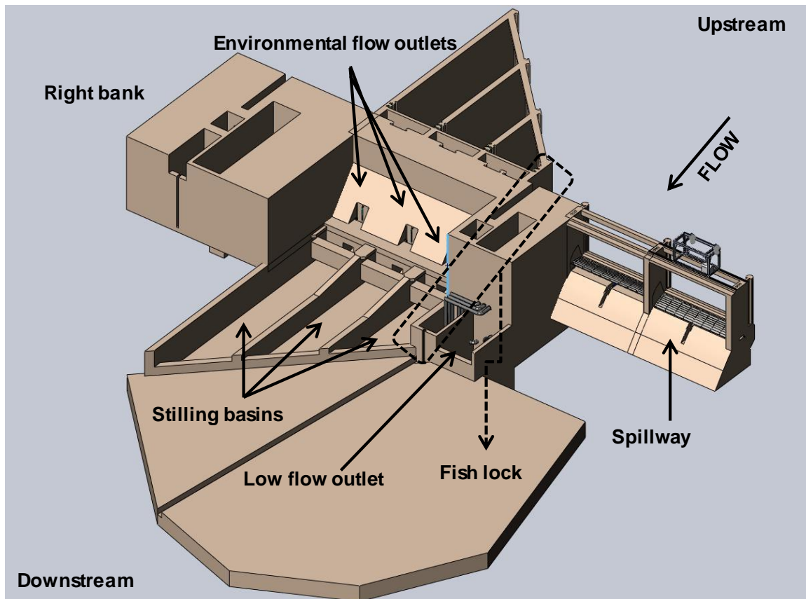
Figure 2-13 Eden Bann Weir right bank outlets and fish lock design
