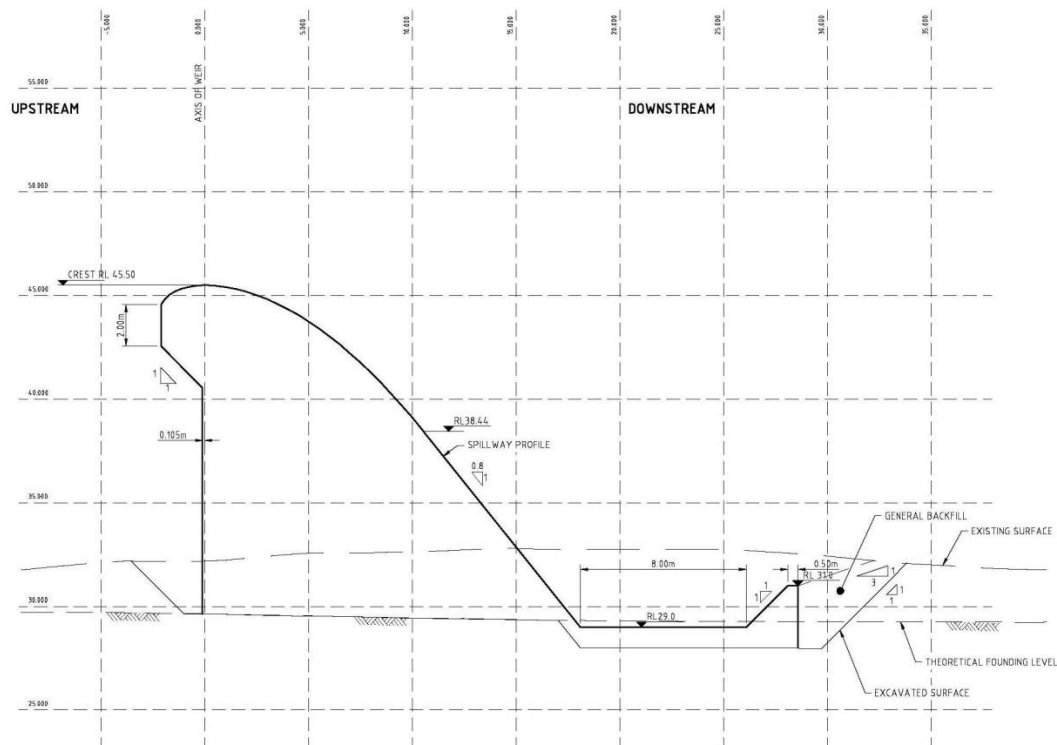
Figure 2-16 Rookwood Weir Stage 2 ogee spillway section
