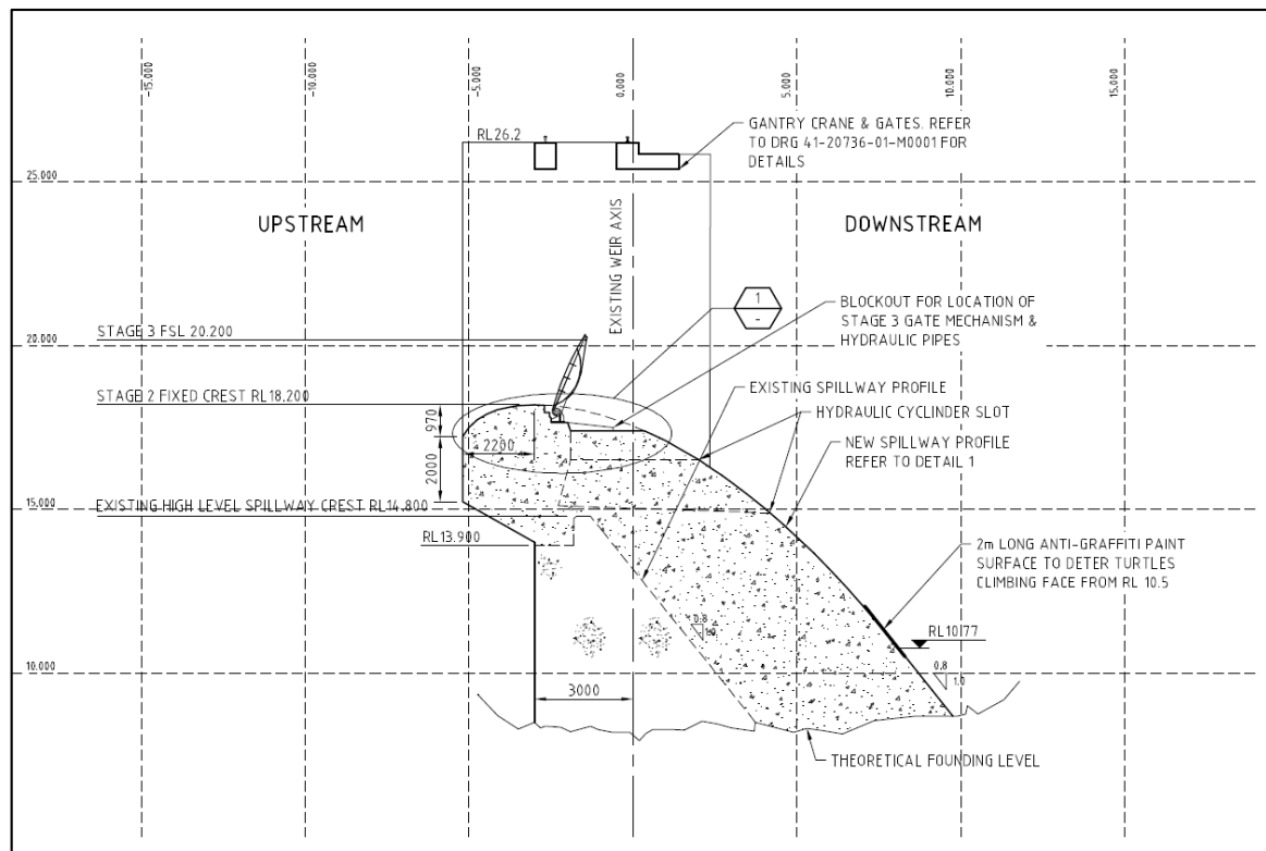
Figure 2-11 Eden Bann Weir Stage 3 ogee (high level) spillway section with flap gates
