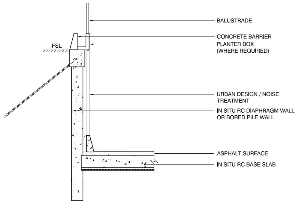
TRANSITION STRUCTURE
