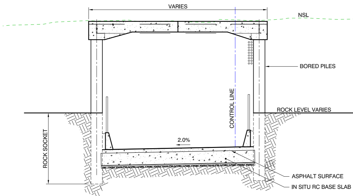
CUT AND COVER TUNNEL
