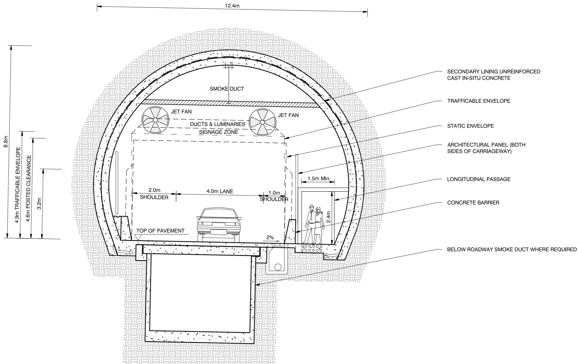
ONE LANE ROADHEADER TUNNEL WITH LONGITUDINAL PASSAGE
