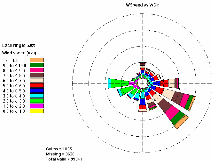
Figure F.1 Direction and frequency of winds at Mackay, October 1995 to June 2007
