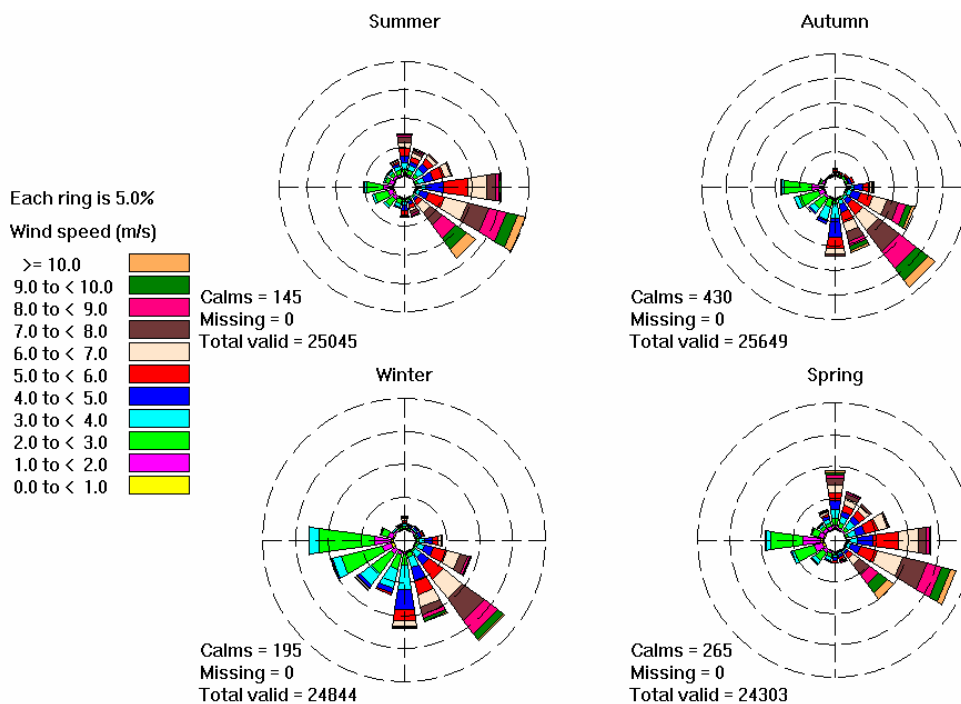
Figure F.2 Direction and frequency of winds during summer (upper left), autumn (upper right), winter (lower left) and spring (lower right) at Mackay, October 1995 to June 2007
