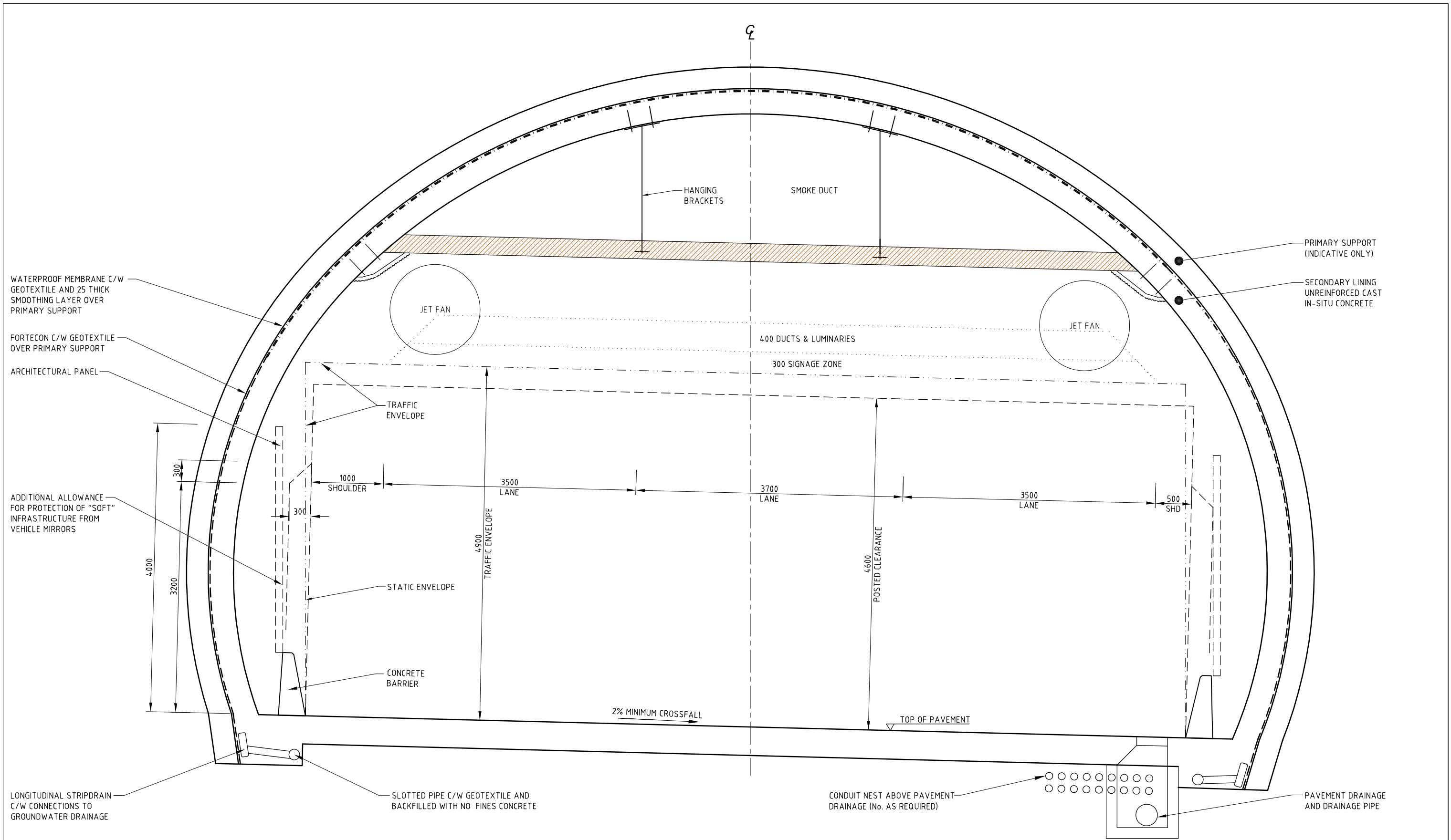
STANDARD THREE LANE ROADHEADER TUNNEL-SECTION
