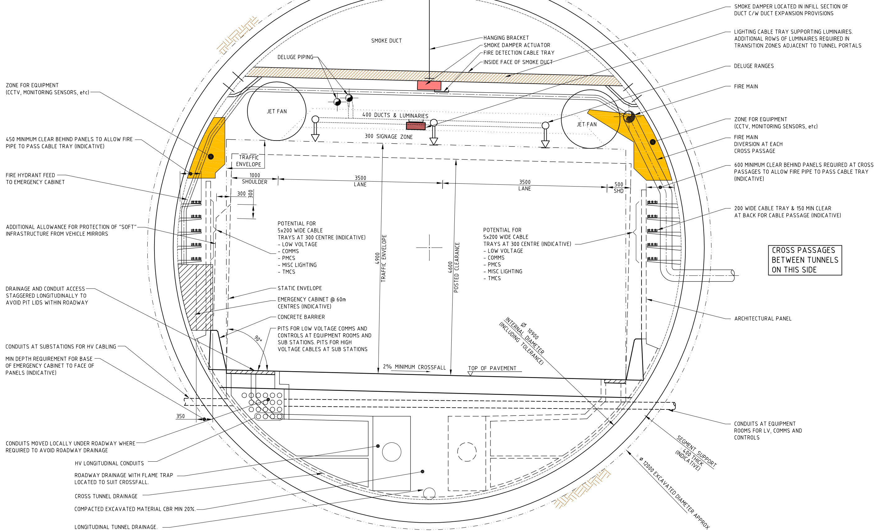
STANDARD TWO LANE TBM (EPBM) TUNNEL-SECTION
